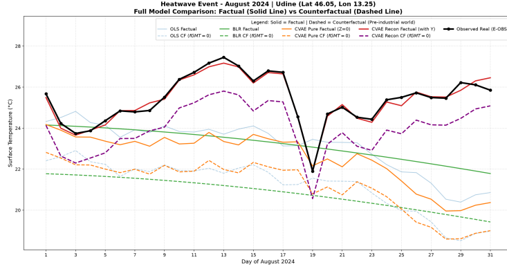
Figure 2: A graph that measures how much hotter the month of August in Udine for the year 2024. The black line representing the observed data shows an increase in the temperatures above 27°C in the middle of the month then begin to gradually decrease at the end of the month. The counterfactual lines of all the models clearly shows a gap between them and the factual lines indicating how lower the temperatures could have been without the presence of pollution.
