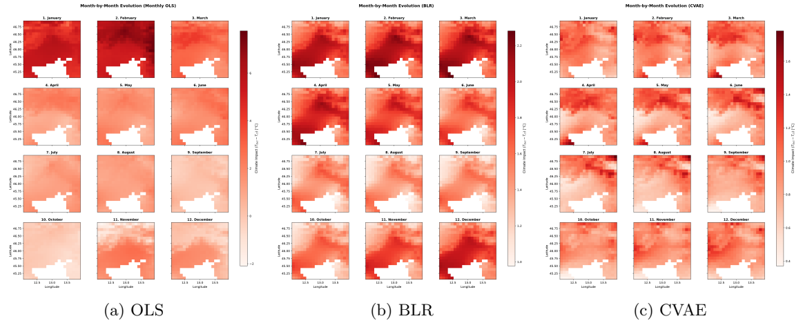
Figure 3: It shows the heat map the Friuli Venezia Giulia for all three models. It shows the spatial evidence of climate-change impact during the months of the year. While the BLR and the CVAE show a smooth and coherent heat map over the time, the OLS is filled with noise. The darker red spots occur more during the winter period showing signs of a more stronger warming while the lighter red ones occur during the summer period with signs of not so strong warming
