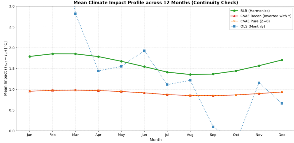
Figure 1: We can notice that BLR and CVAE have a sinusoidal pattern. That means that the climate impact sensitivity has a seasonal pattern. On the other hand, the OLS model does not capture this trend. The OLS graph shows to include a lot of noise. While the BLR captures a more realistic seasonal cycle the CVAE shows a more stable but smooth pattern cycle.
