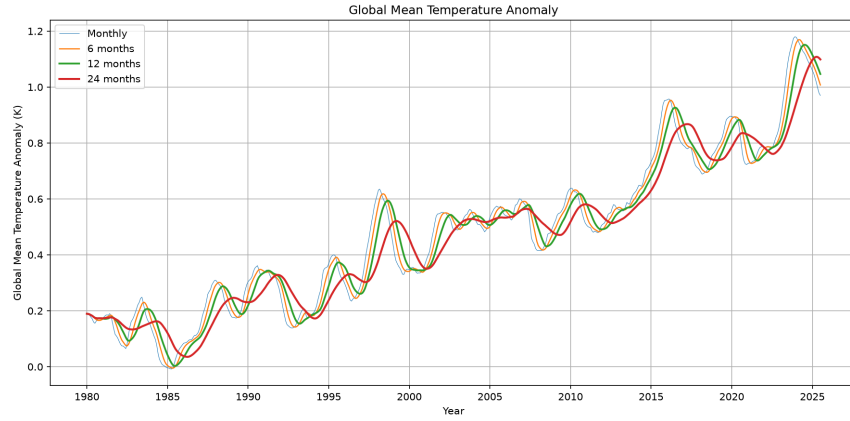
Figure 5: It shows a clear long-term increase in global mean temperature anomaly from the 1980s to 2025. The monthly series contains more short-term fluctuations, while the 6-, 12- and 24-month moving averages progressively smooth these variations. The 12-month series provides a good compromise between reducing short-term noise and preserving the main evolution of the global warming signal, which is why it was selected for the main analysis.
