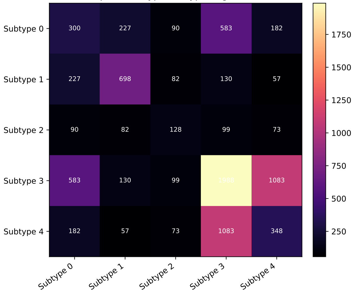
Graph 2: subtype-subtype edge counts
