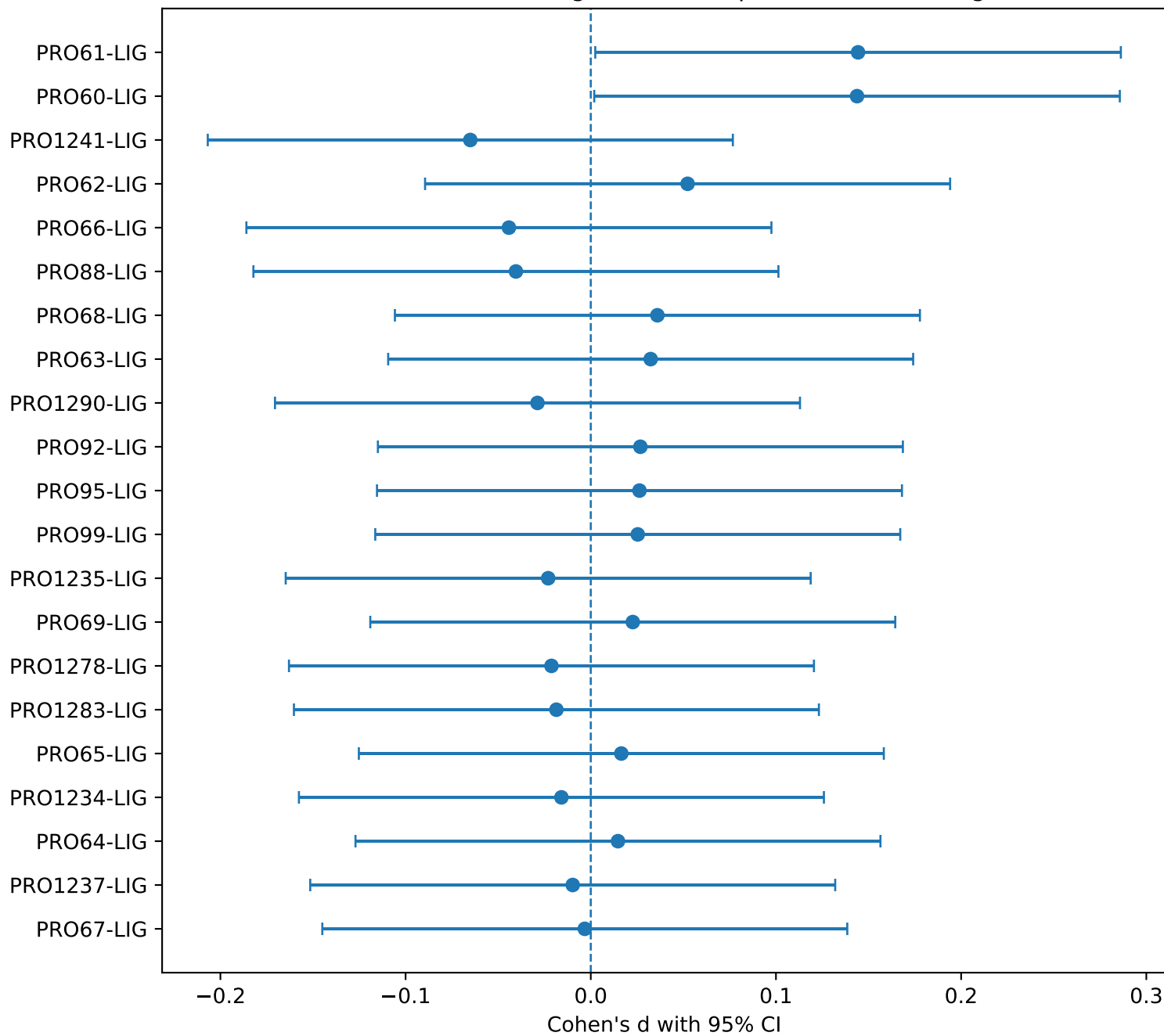
PRO-LIG differences: high vs low RF-predicted barrier ligands
