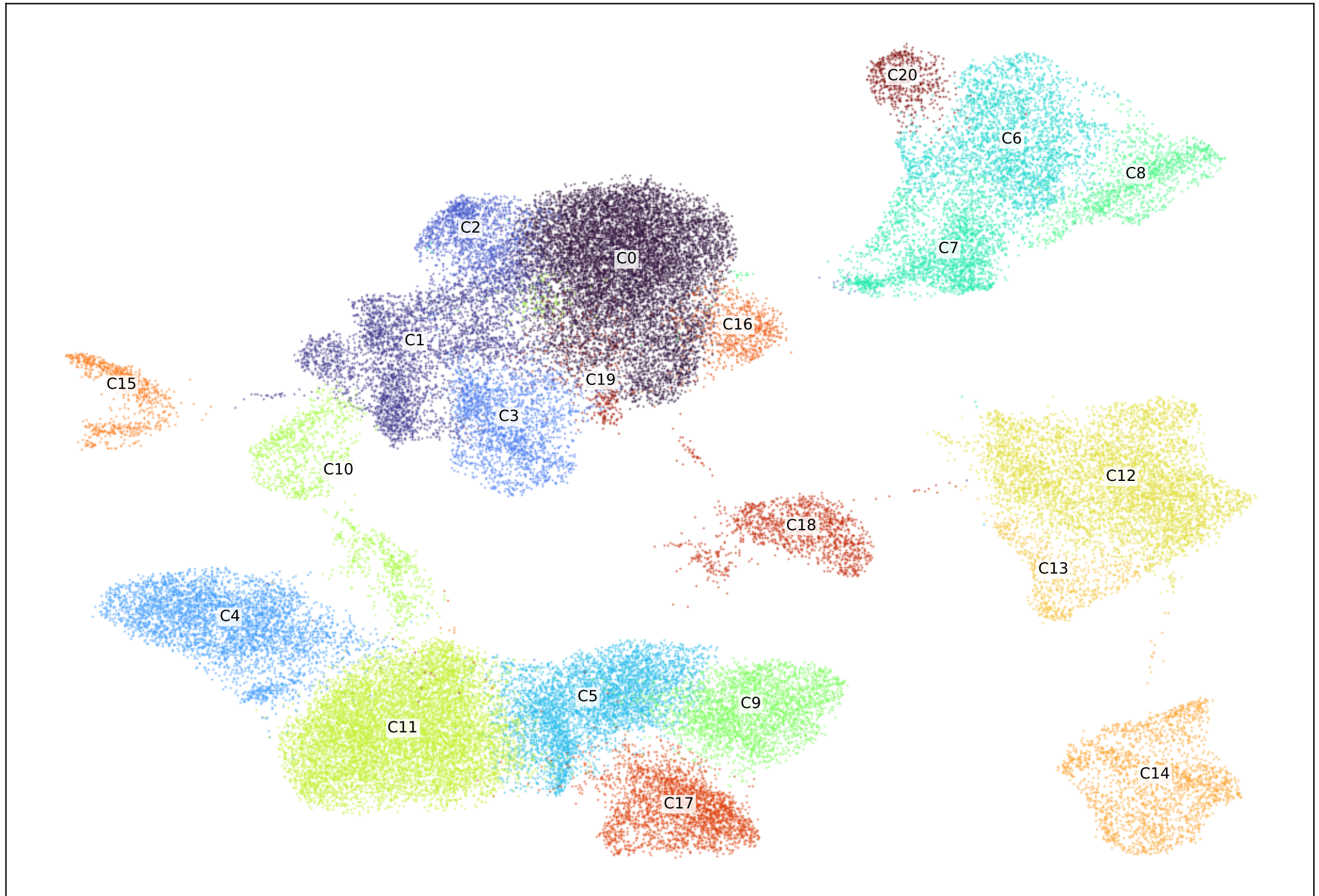
GSE202642 | 7 HCC tumor samples | Harmony + Leiden
