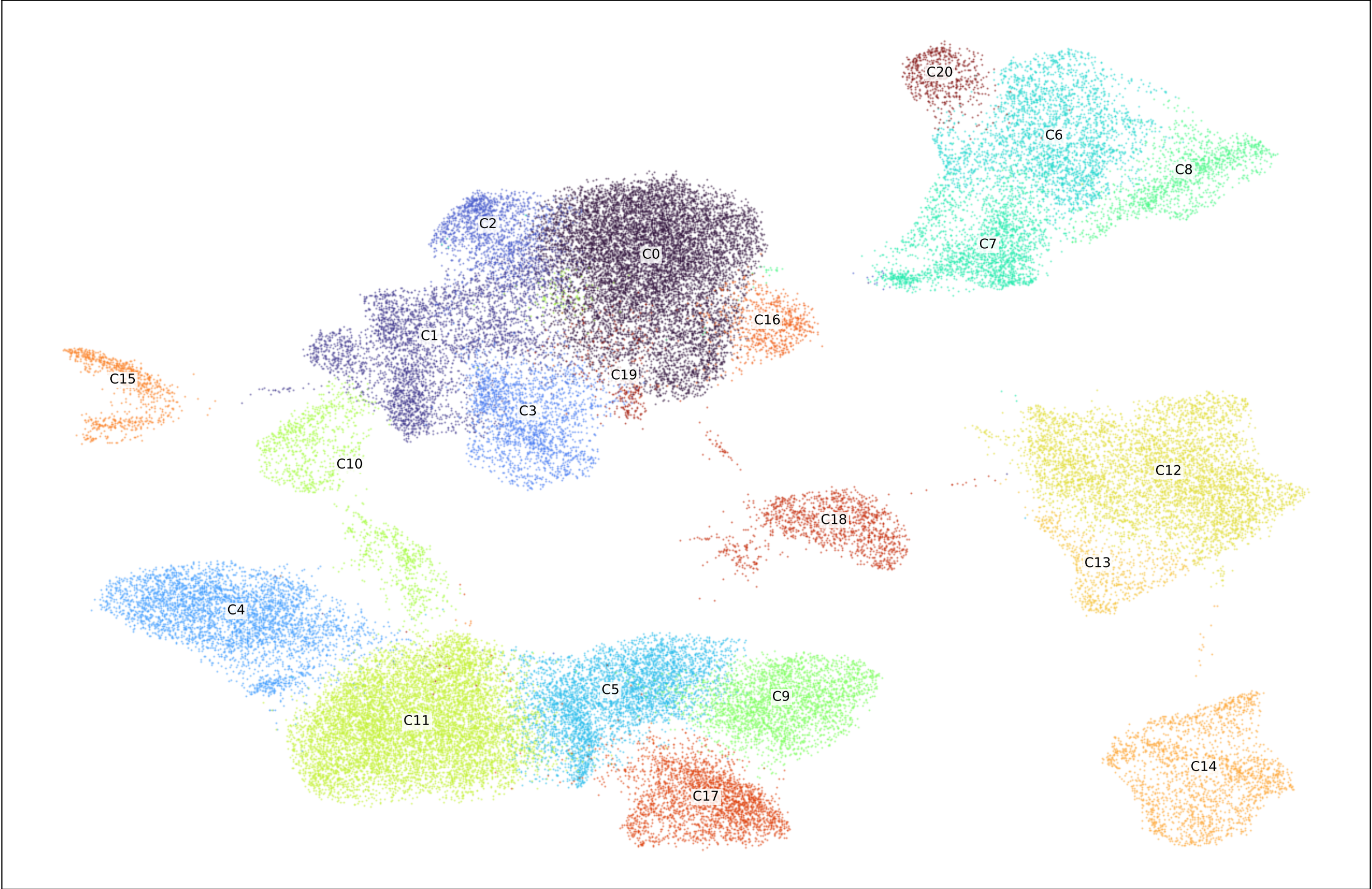
GSE202642 | 7 HCC tumor samples | Harmony + Leiden
