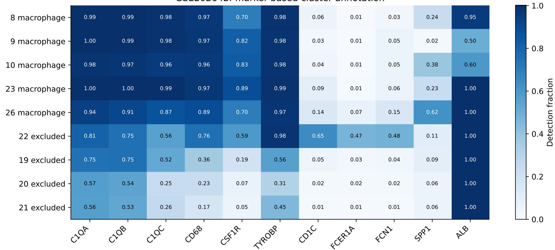
GSE202642: marker-based cluster annotation
