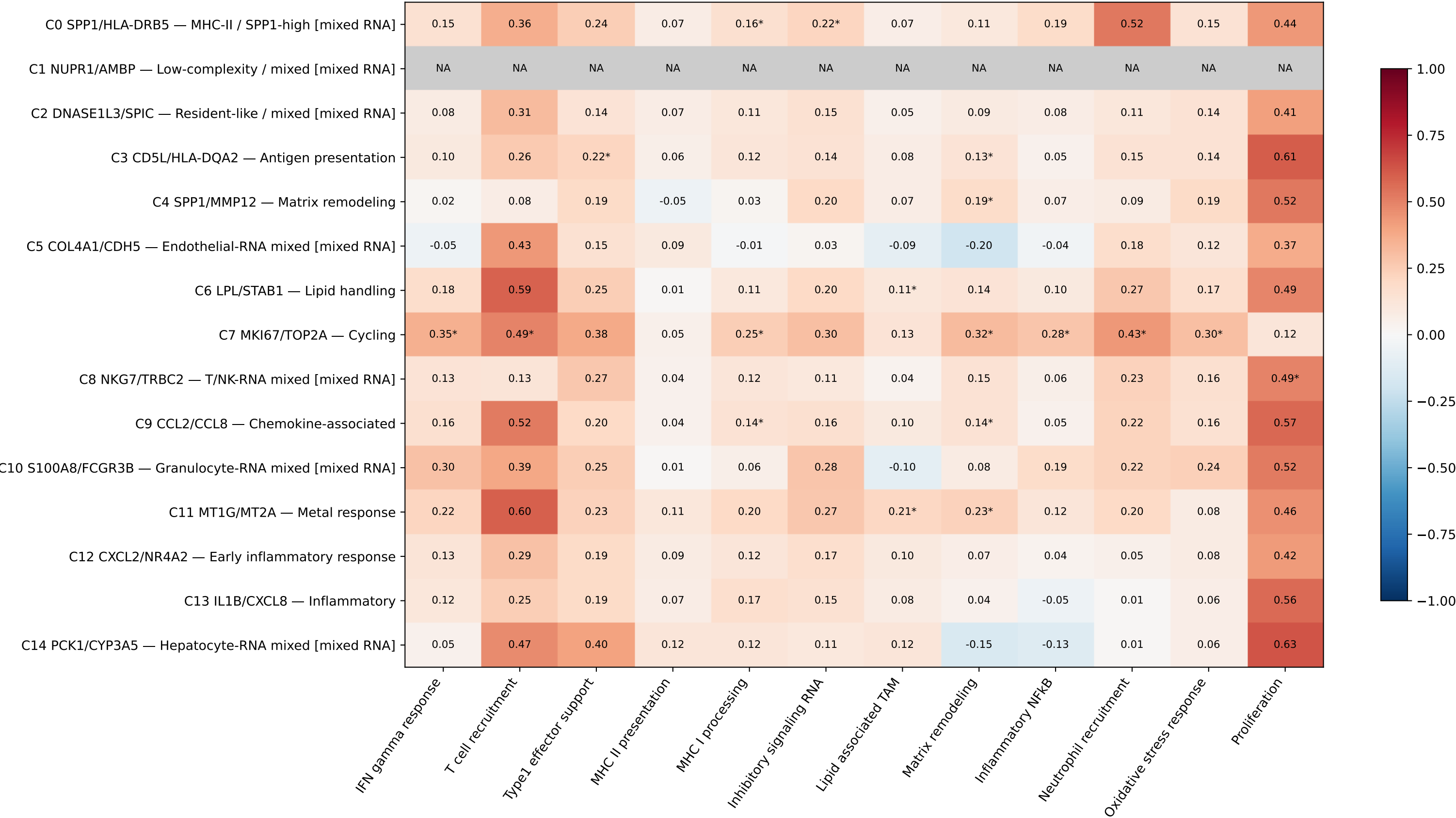
Observed Spearman rho (PGAM5 included in every score)
