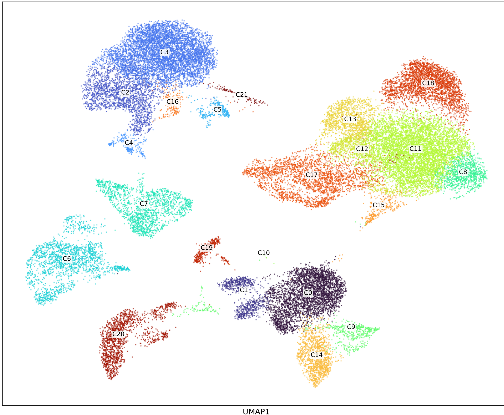
GSE149614 HCC | cluster labels
