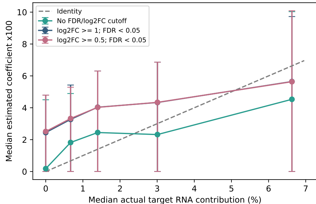
Observed-library RNA mixtures
