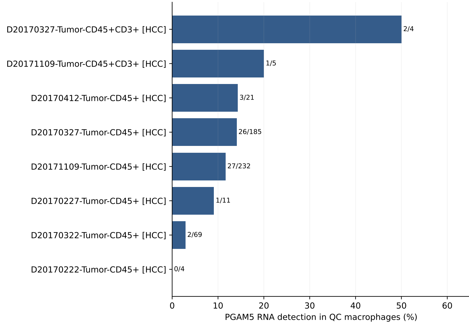
Smartseq2
