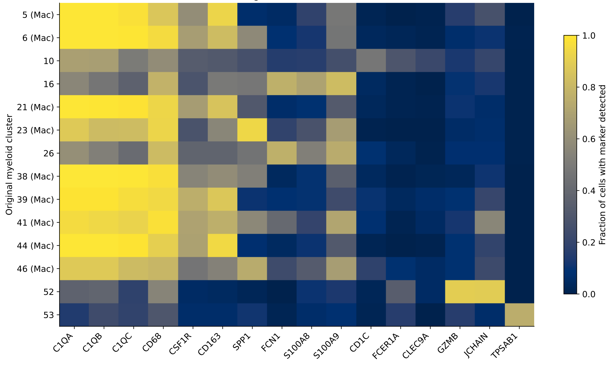
GSE149614 original clusters: marker detection
