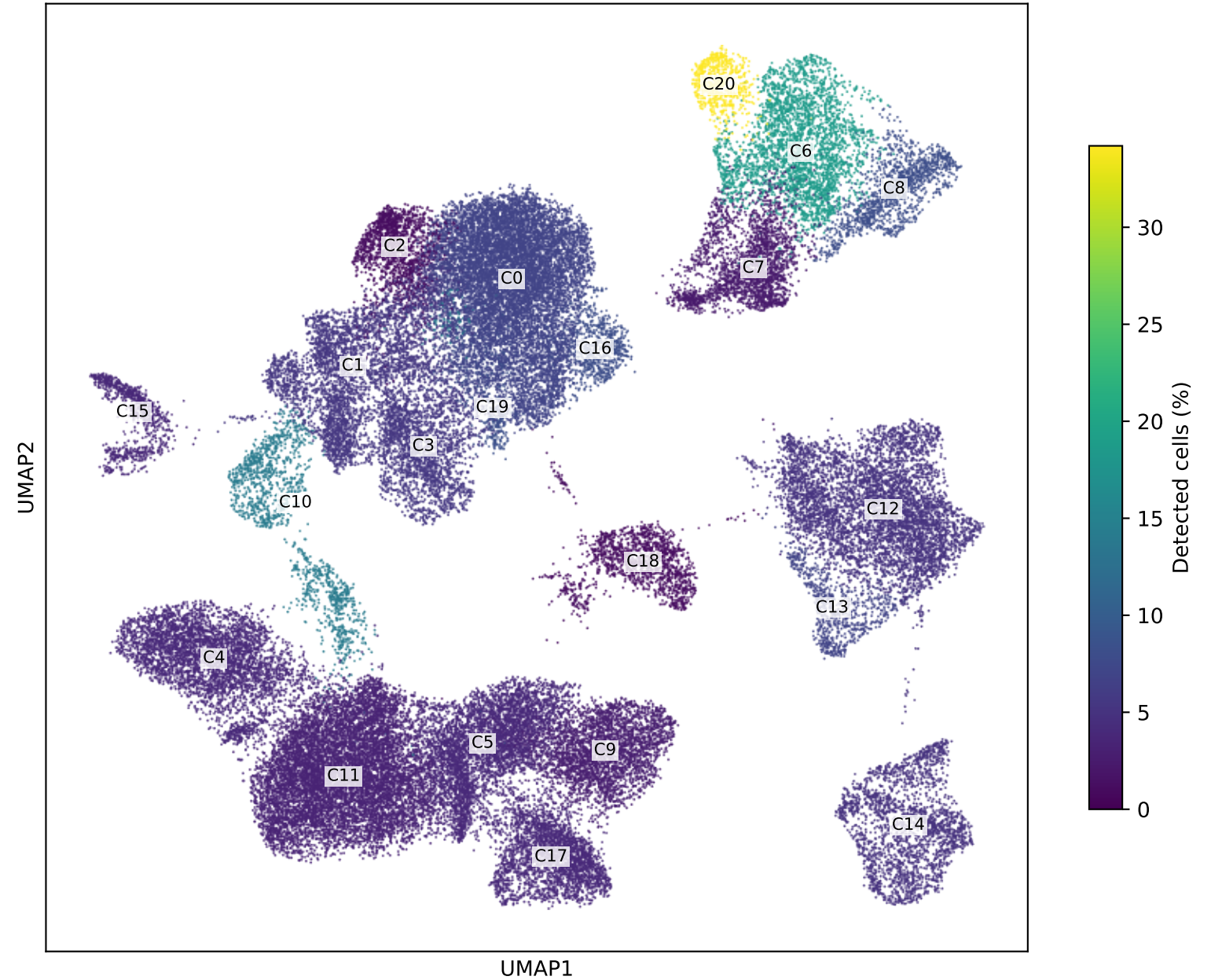
Cluster PGAM5 RNA detection rate
