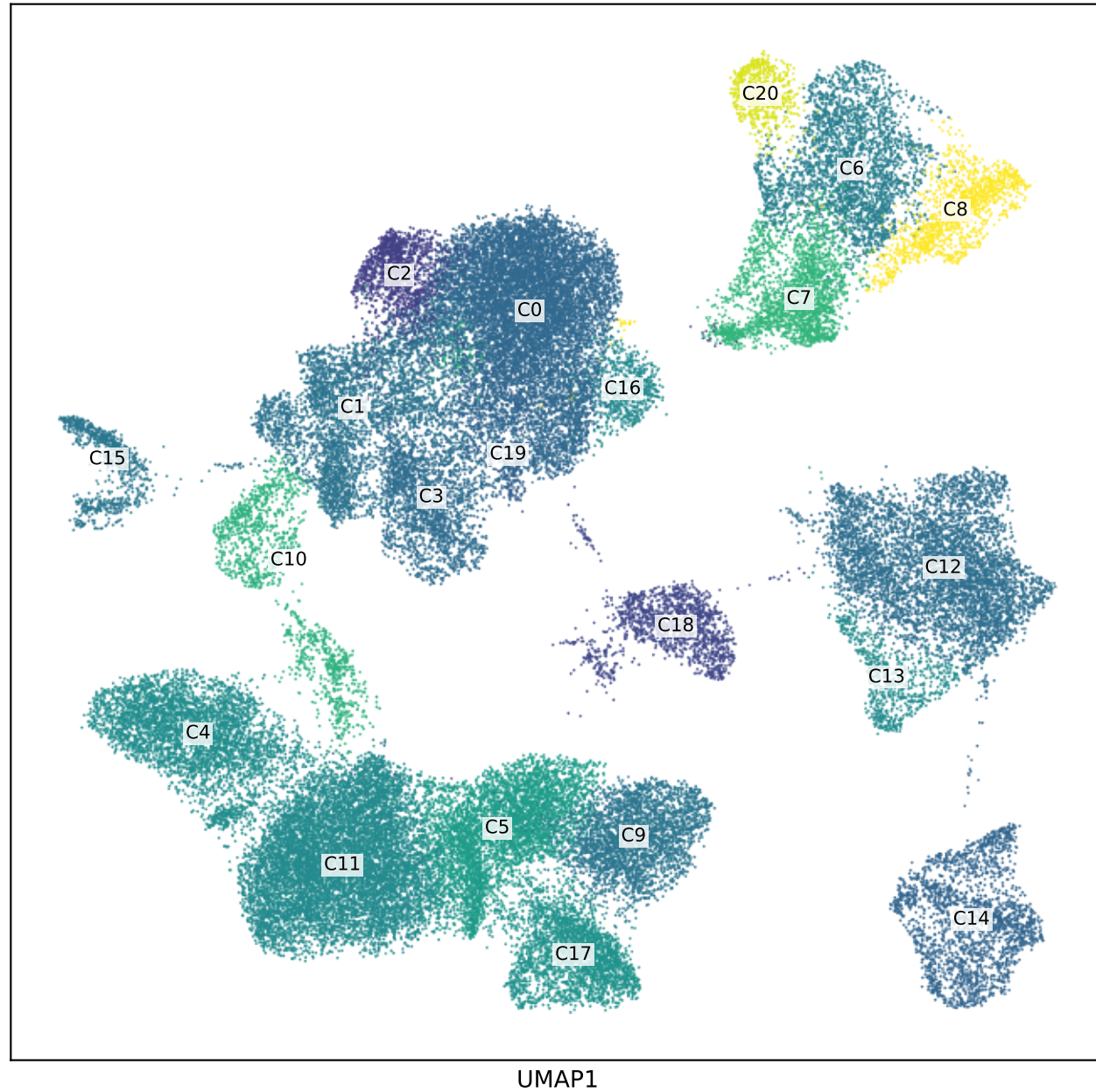
Cluster mean PGAM5 expression (zeros included)
