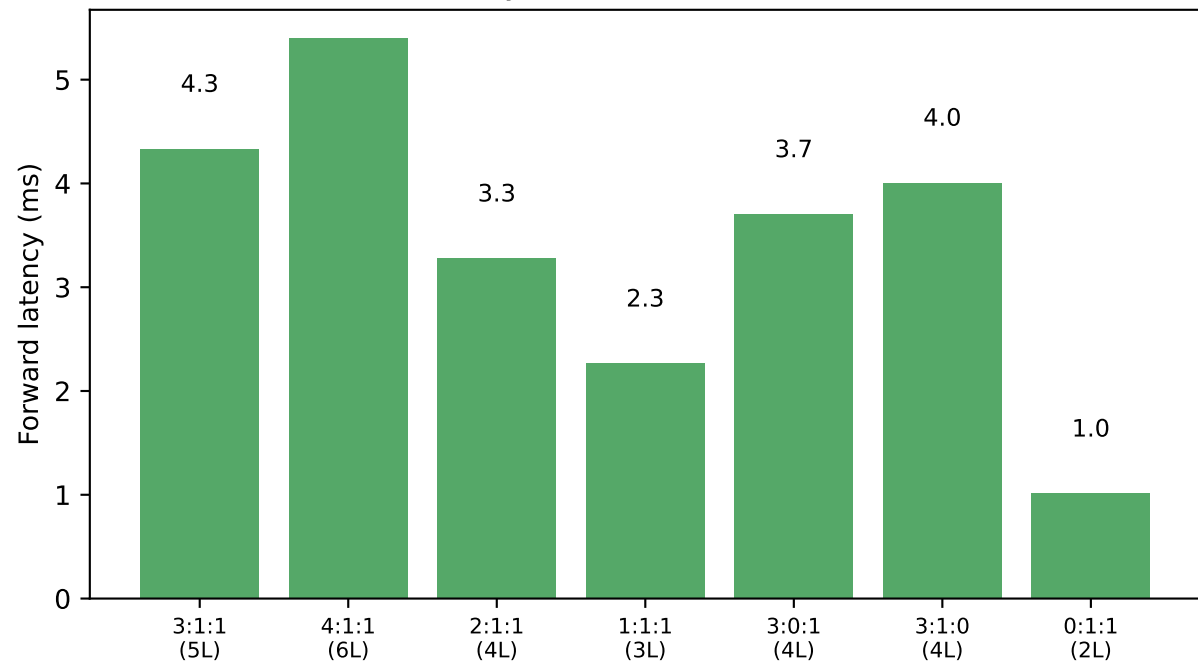
5.4 Latency vs. KDA:CSA:HCA ratio
