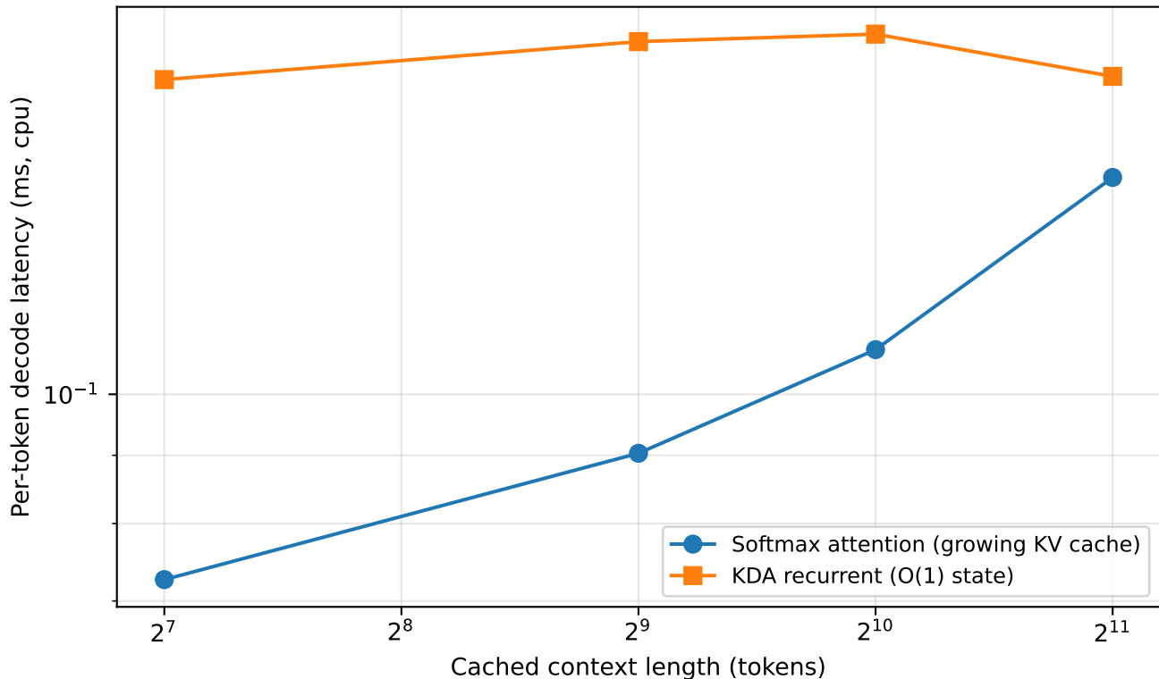
Decoding latency vs. cached context length
