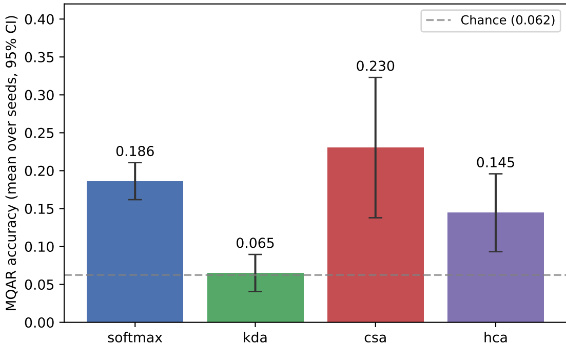
Multi-Query Associative Recall ( n_{kv}=1 , 3 seeds, 200 steps)
