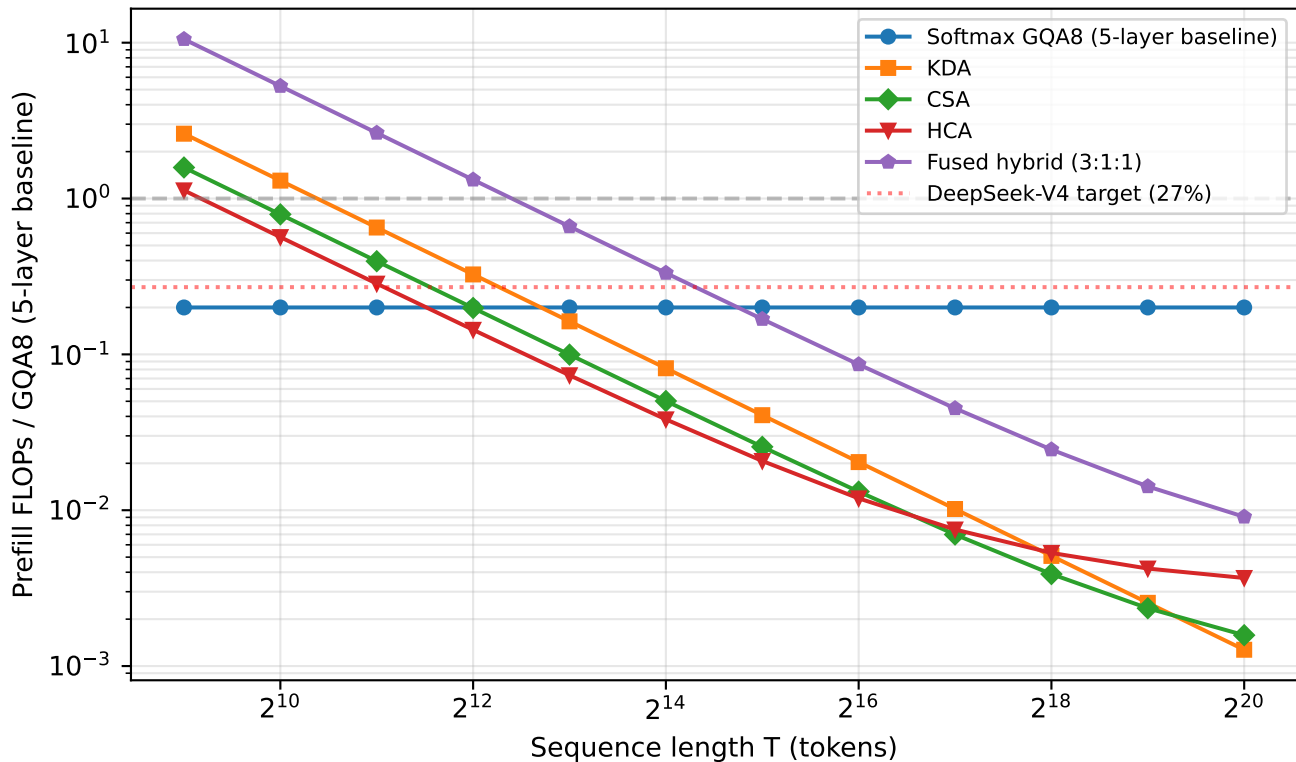
Prefill compute vs. sequence length
