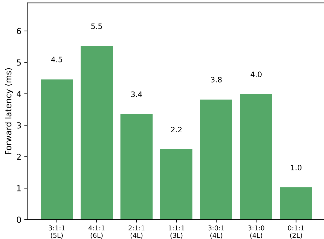
Latency vs. KDA:CSA:HCA ratio
