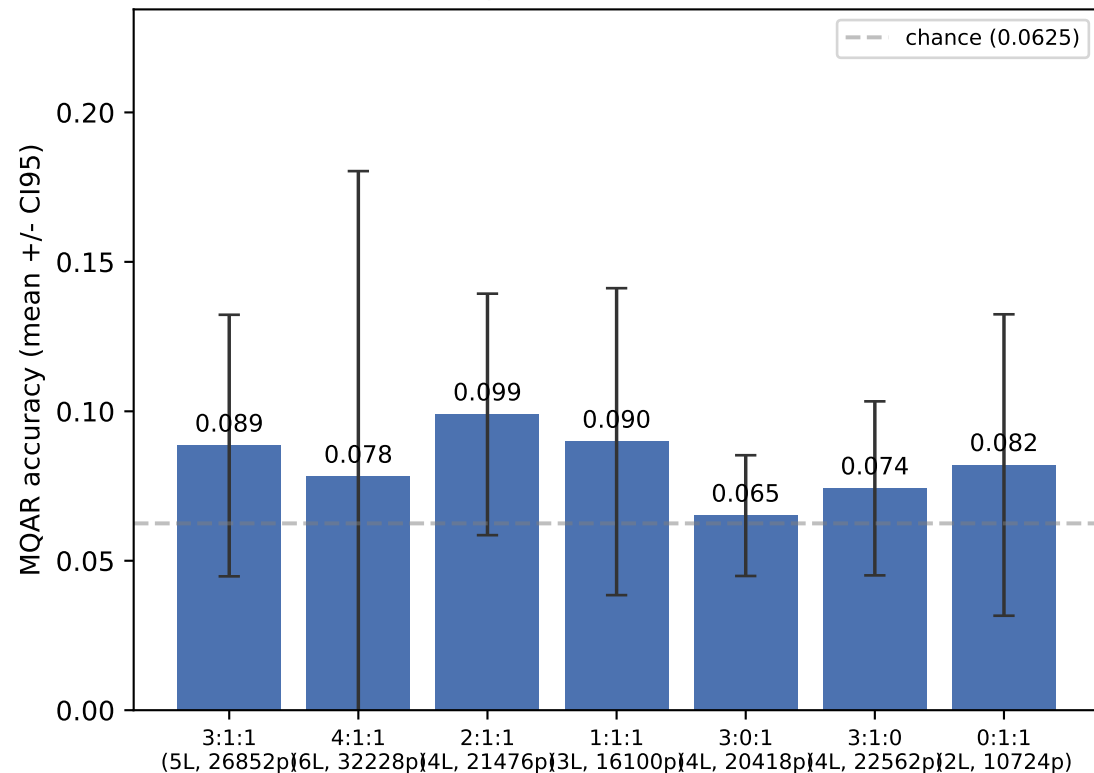
Accuracy vs. KDA:CSA:HCA ratio
