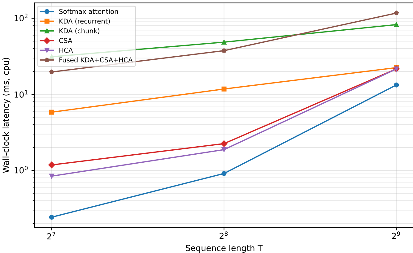
Operator latency vs. sequence length
