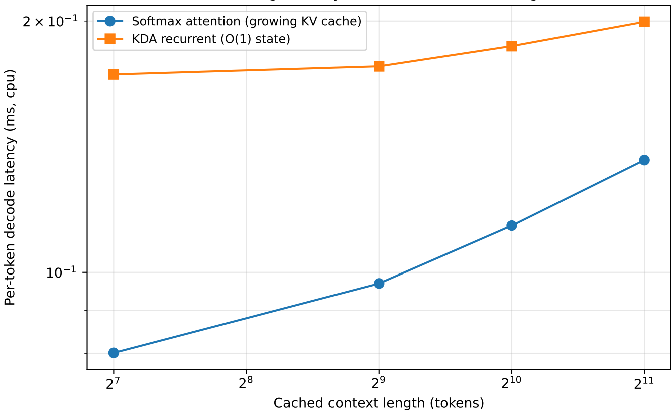
Decoding latency vs. cached context length
