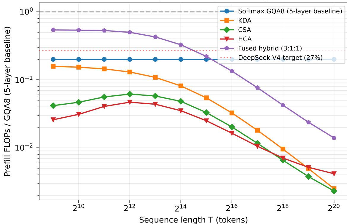
Prefill compute vs. sequence length
