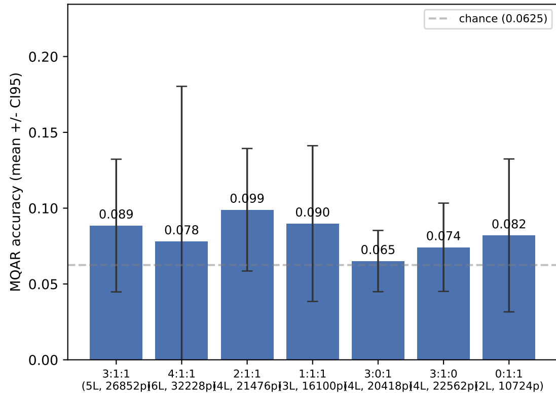
Ablation: ratio trade-off ( n_{kv}=1 , multi-seed). 4:1:1 has 6L vs 0:1:1 has 2L — depth confound noted in paper. Accuracy vs. KDA:CSA:HCA ratio
