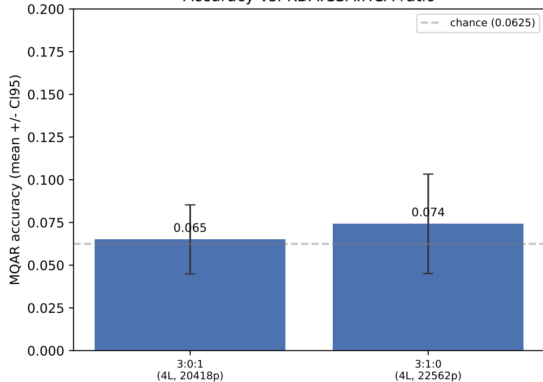
Accuracy vs. KDA:CSA:HCA ratio
