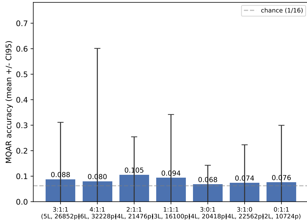
Ablation: ratio trade-off ( n_{kv}=1 , multi-seed). 4:1:1 has 6 layers vs 3:1:1 has 5 — depth confound noted in paper. Accuracy vs. KDA:CSA:HCA ratio
