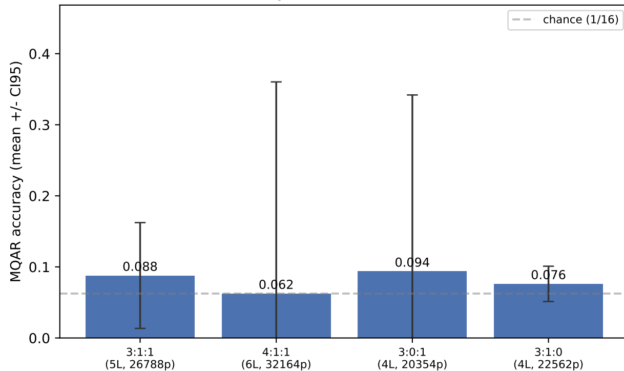
Accuracy vs. KDA:CSA:HCA ratio
