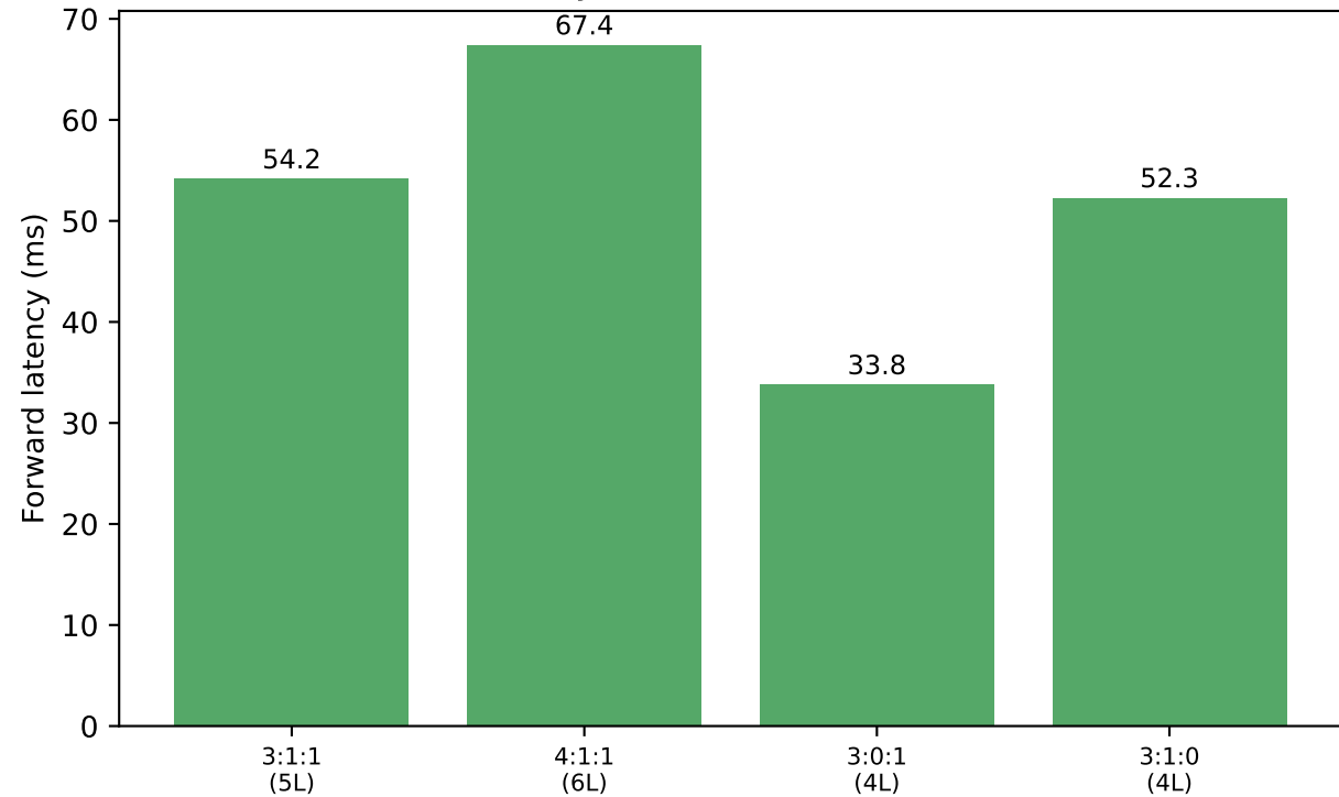
Latency vs. KDA:CSA:HCA ratio
