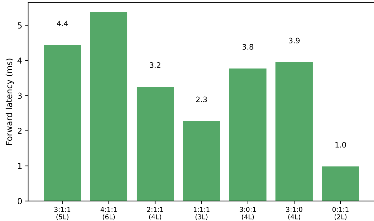
5.4 Latency vs. KDA:CSA:HCA ratio
