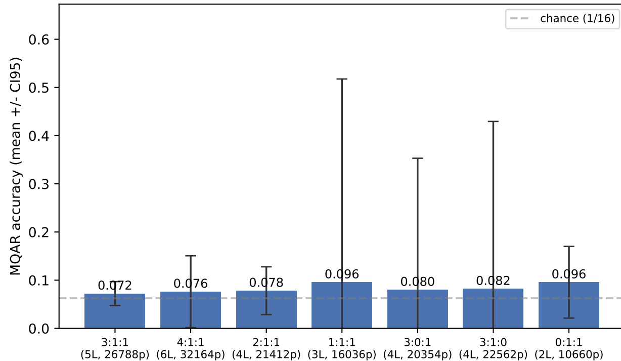
Accuracy vs. KDA:CSA:HCA ratio
