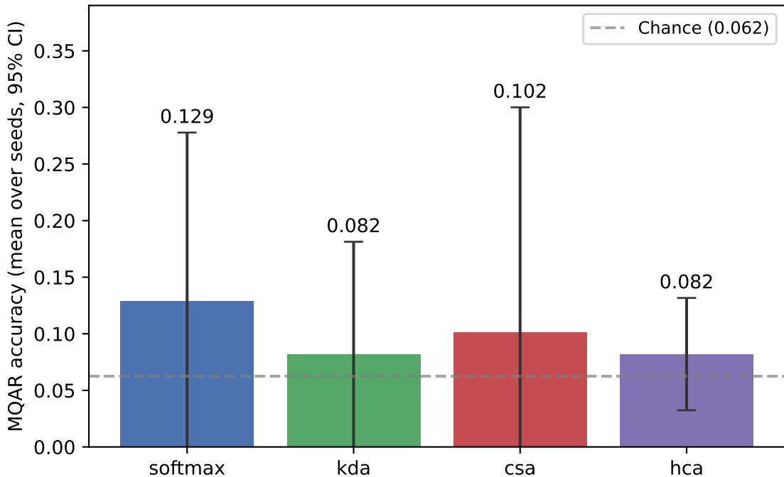
Multi-Query Associative Recall (n_kv=1, 2 seeds, 100 steps)
