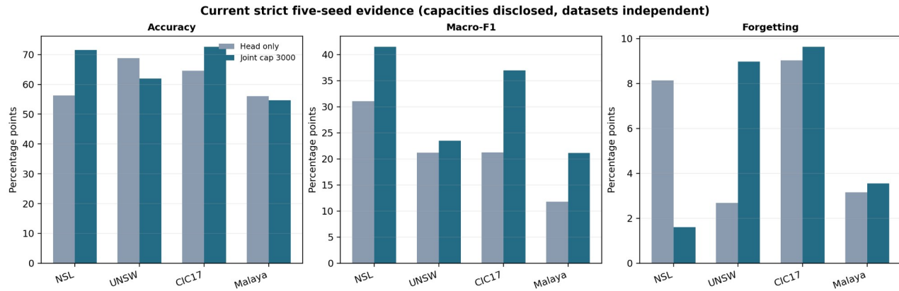
Figure 2. Head-only versus joint-cap current strict five-seed means. Capacities are disclosed by dataset and are not pooled.
