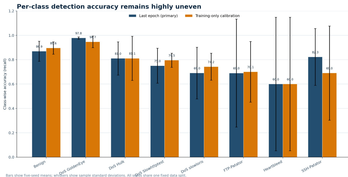
Figure 4. Per-class official joint-cap-3,000 recall. Whiskers are sample standard deviations across five seeds on one fixed split.
