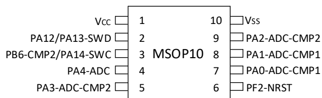
图 3-11 MSOP10 PY32F003A1xNx ( Top view )
