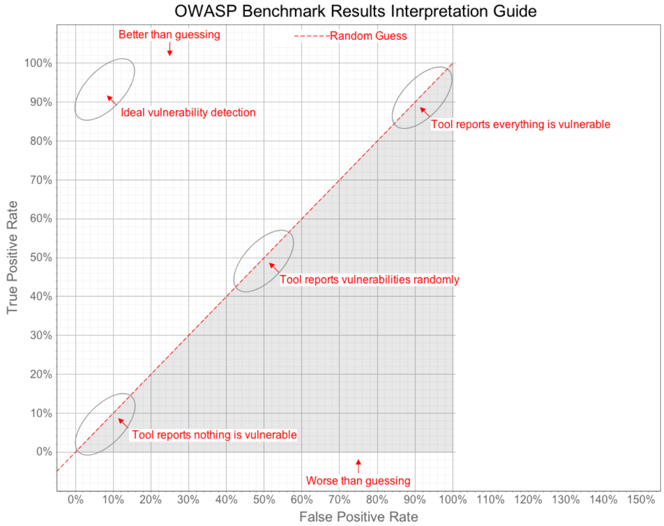
Fig. 1: OWASP Benchmark Scoring Guide - Youden Index interpretation [31]
