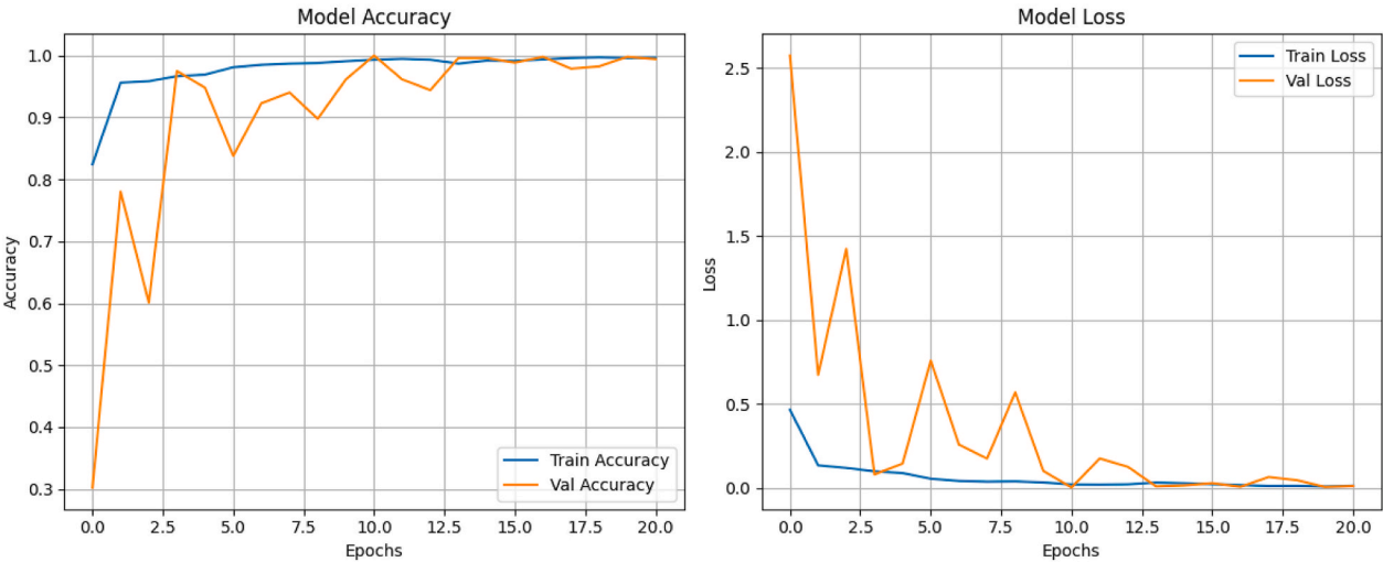
(b) VGG16
