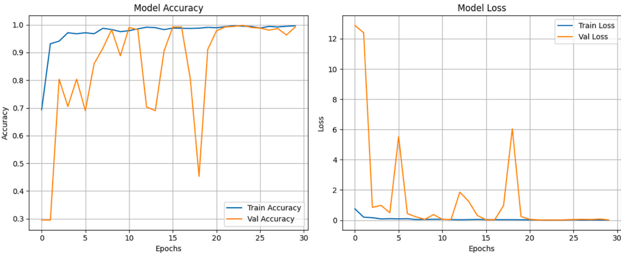
(c) VGG19
