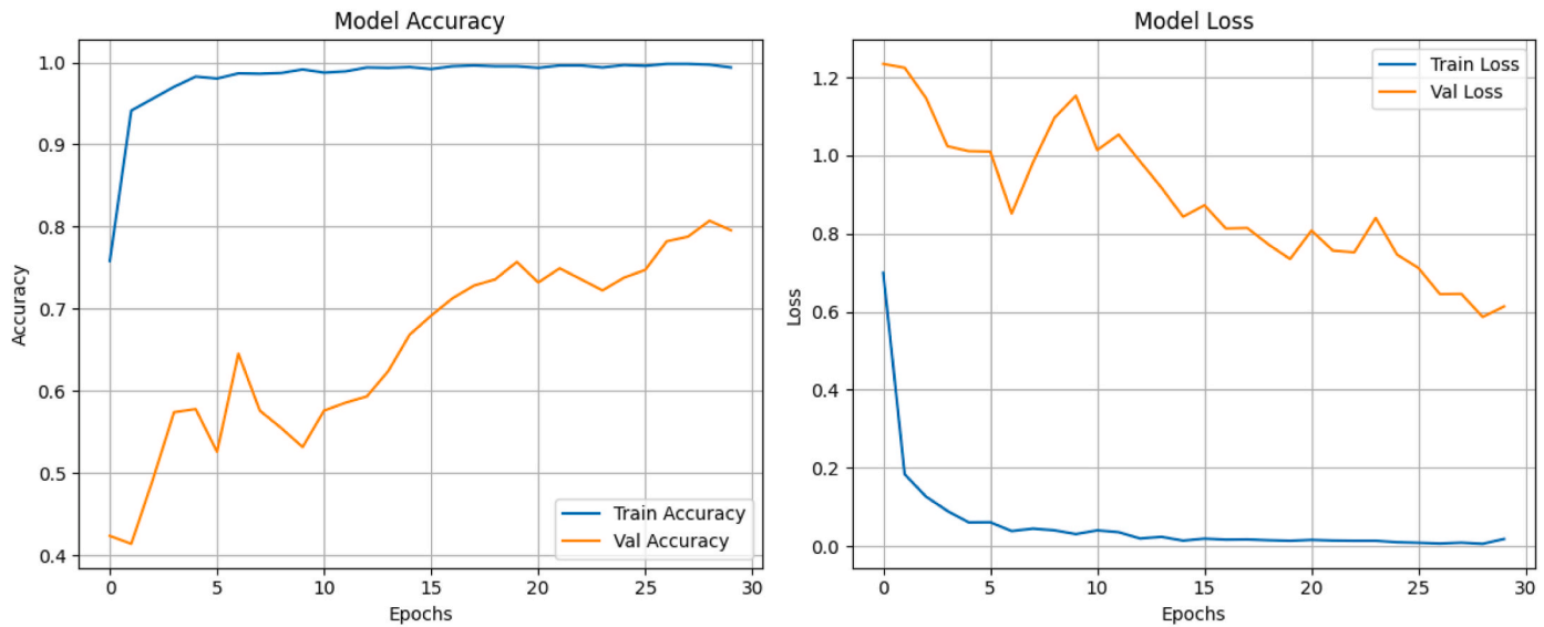
(a) NASNetMobile
