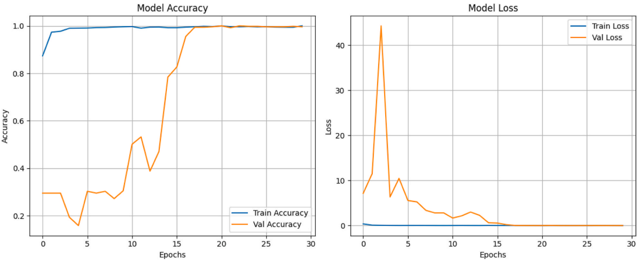
(a) ResNet50
