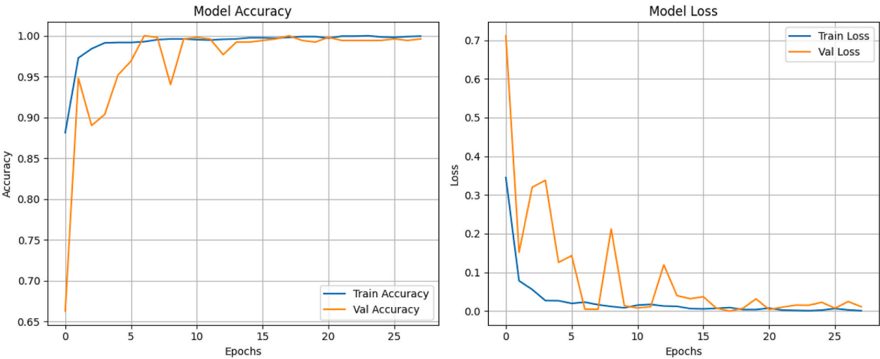
(a) DenseNet 169
