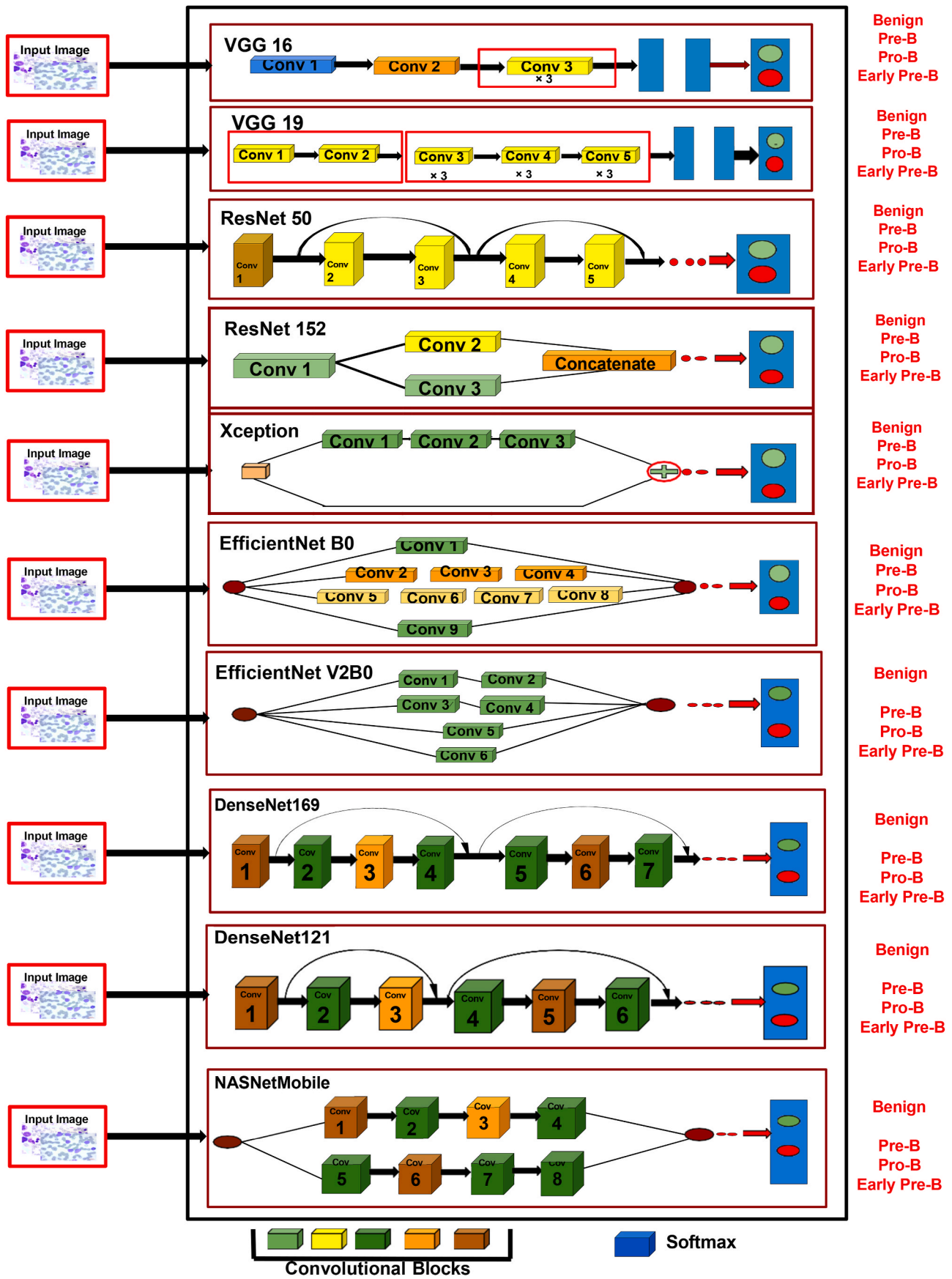
Fig. 2. Proposed model.
