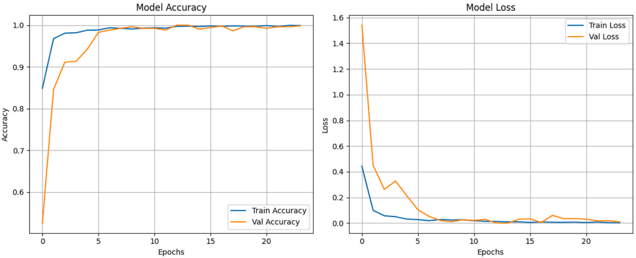
(c) DenseNet 121
