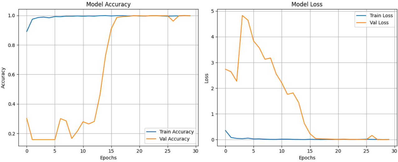
(b) ResNet152
