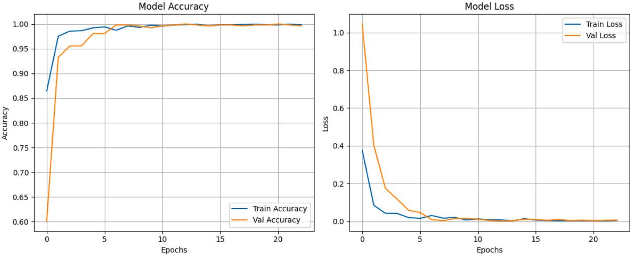
(c) Xception
