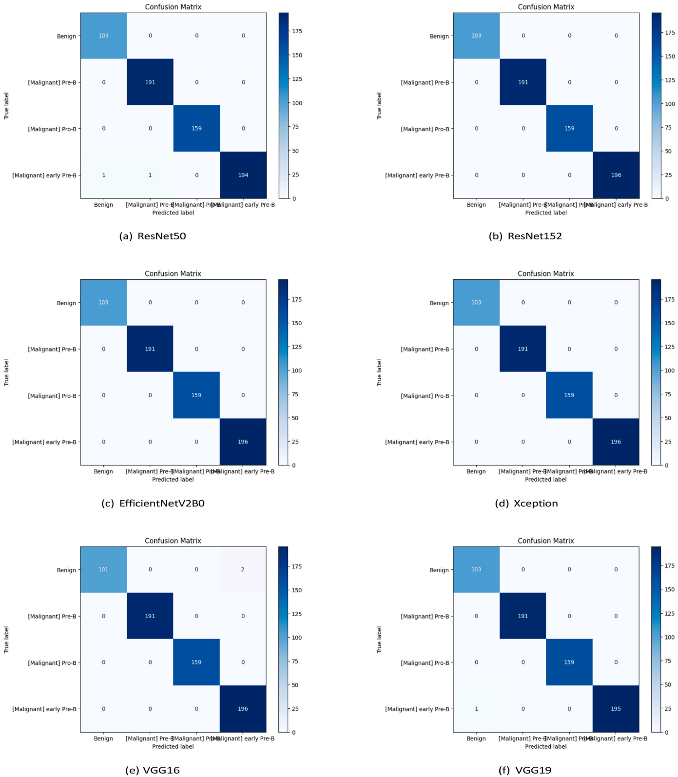
Fig. 12. Model architecture confusion Matrices 2.
