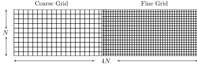
Figure 10: Setup for the channel flow
