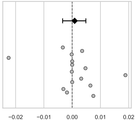
Pixel AP
