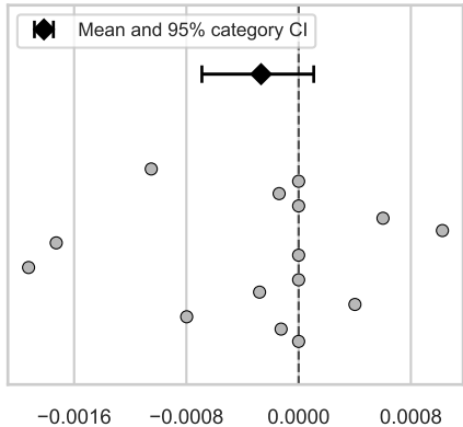
Image AUROC
