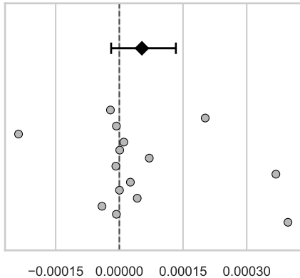
Pixel AUROC
