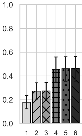
Pixel AP
