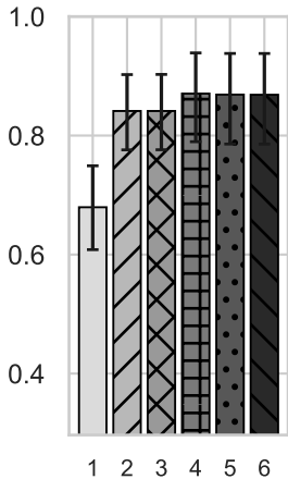
Image AUROC
