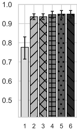
Pixel AUROC
