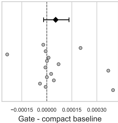
Pixel AUROC
