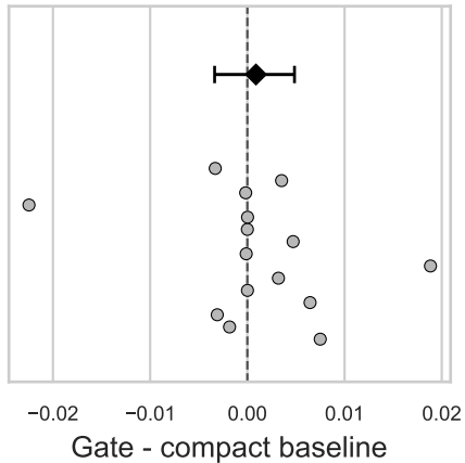
Pixel AP
