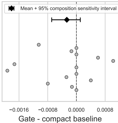
Image AUROC
