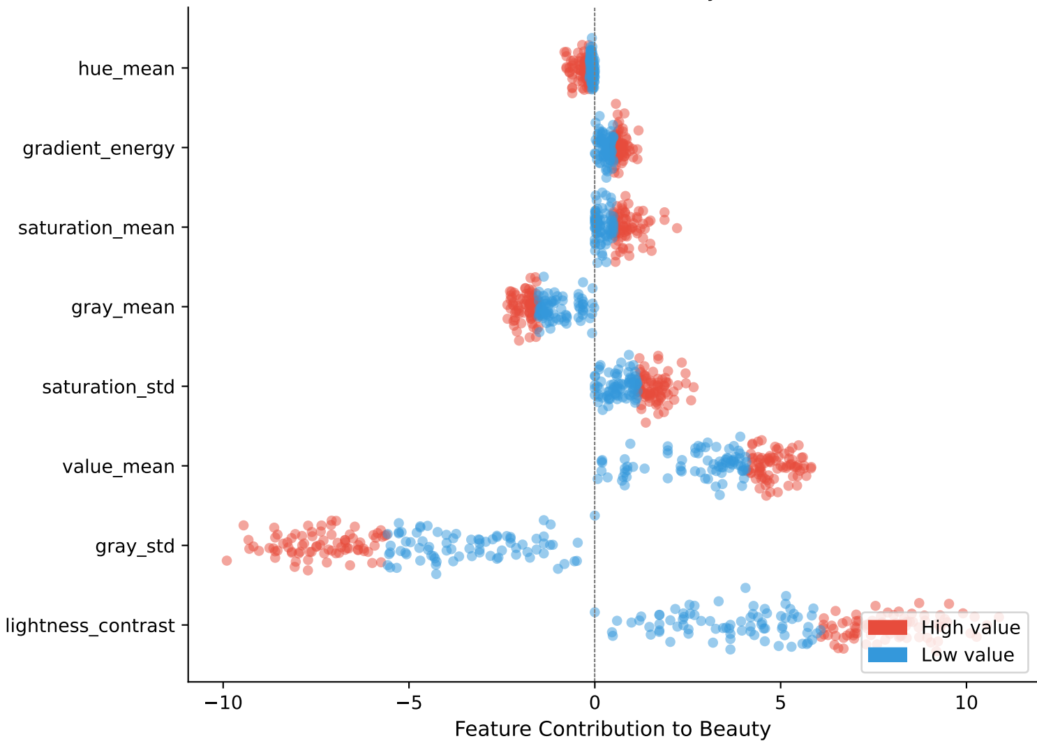
SHAP Beeswarm Plot: Beauty (Phase 2)
