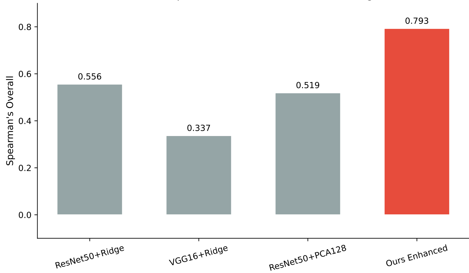
SOTA Comparison (Phase 2, N=160 human ratings)
