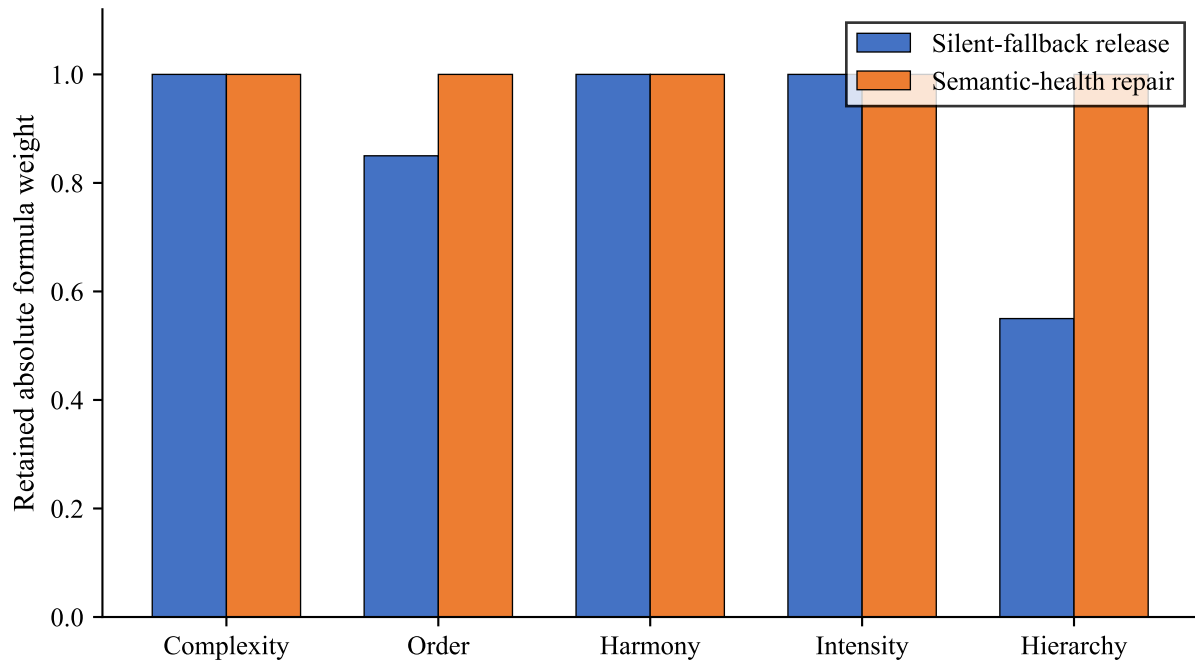
Semantic health exposes inactive weighted features
