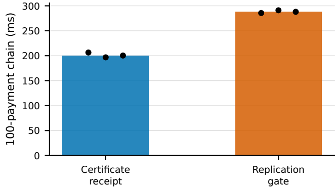
(b) Real consecutive spending; 3 chains
