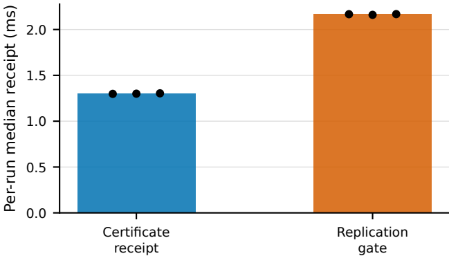
(a) Matched 200 TPS; 3 runs per mode
