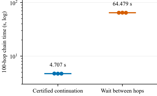
Fig. 4. Current-build 100-hop chains on f856c7b , including client timing probes: three runs per mode, synchronous members and NoSync wallets. Dots are run totals; bars mark medians. Only wait mode requires public observation between hops.
