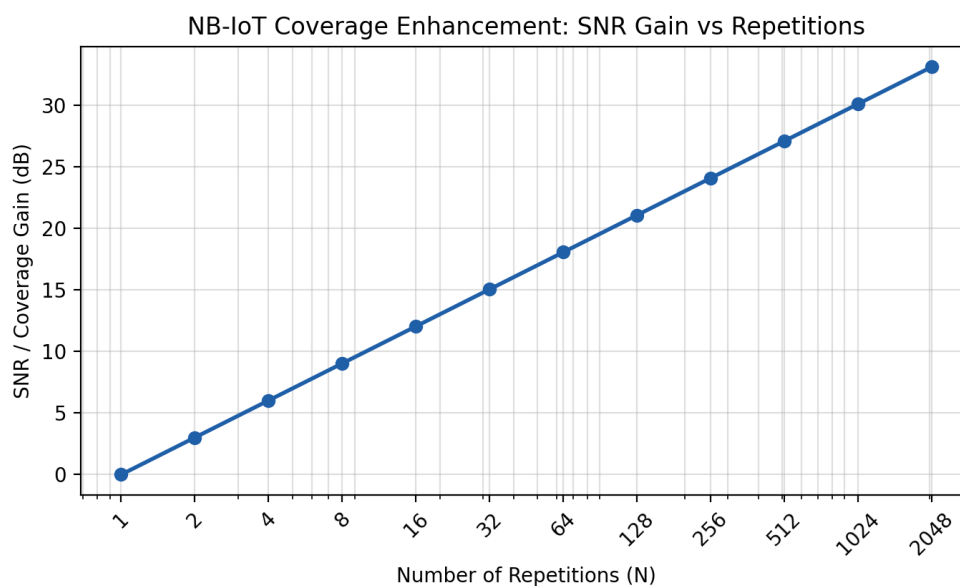
Figure 2: SNR / coverage gain versus number of repetitions
