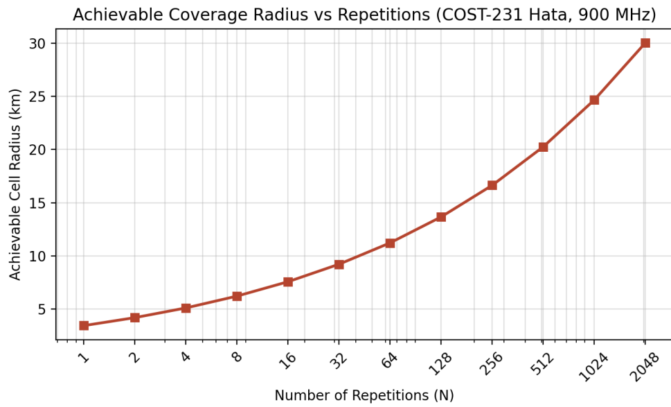
Figure 3: Achievable cell radius versus number of repetitions (COST-231 Hata, 900 MHz)
