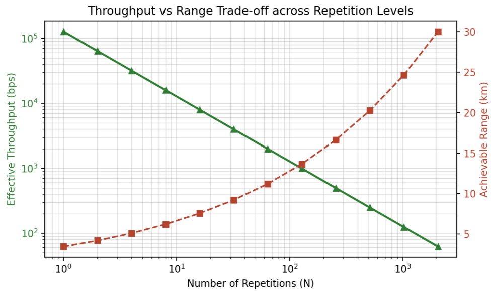
Figure 4: Effective throughput and range trade-off across repetition levels
