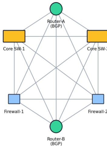
Figure 2: Bank Network
