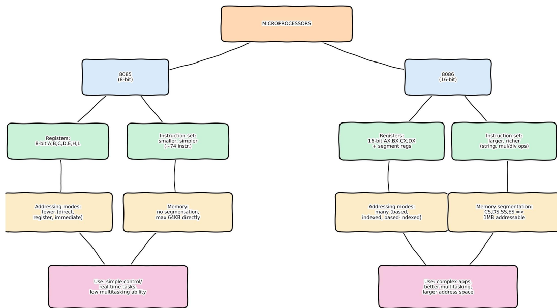
Q3: 8085 vs 8086 Architecture Comparison
