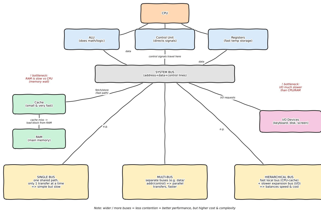
Q1: CPU - Memory - I/O and Bus Structures
