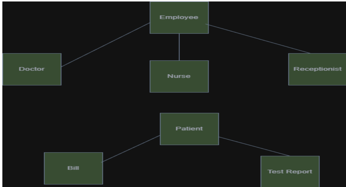
Hospital Management System EER Diagram
