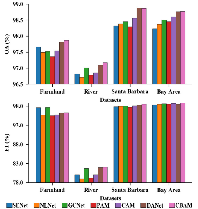
Fig. 10. Accuracy (in terms of OA and F1) of different attention mechanisms.
