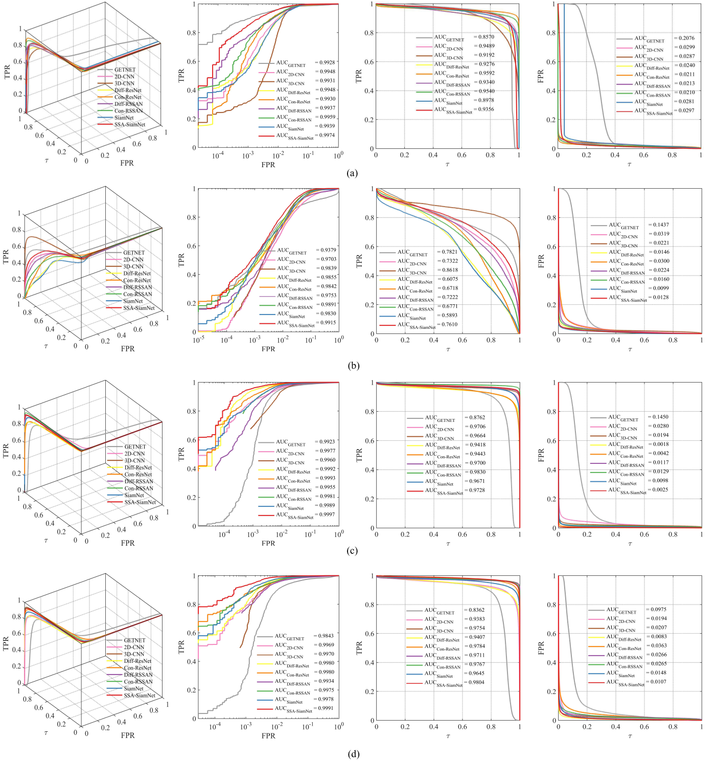
Fig. 3. 3-D ROC curves of different methods for the four datasets. (a) Farmland dataset. (b) River dataset. (c) Santa Barbara dataset. (d) Bay Area dataset.
