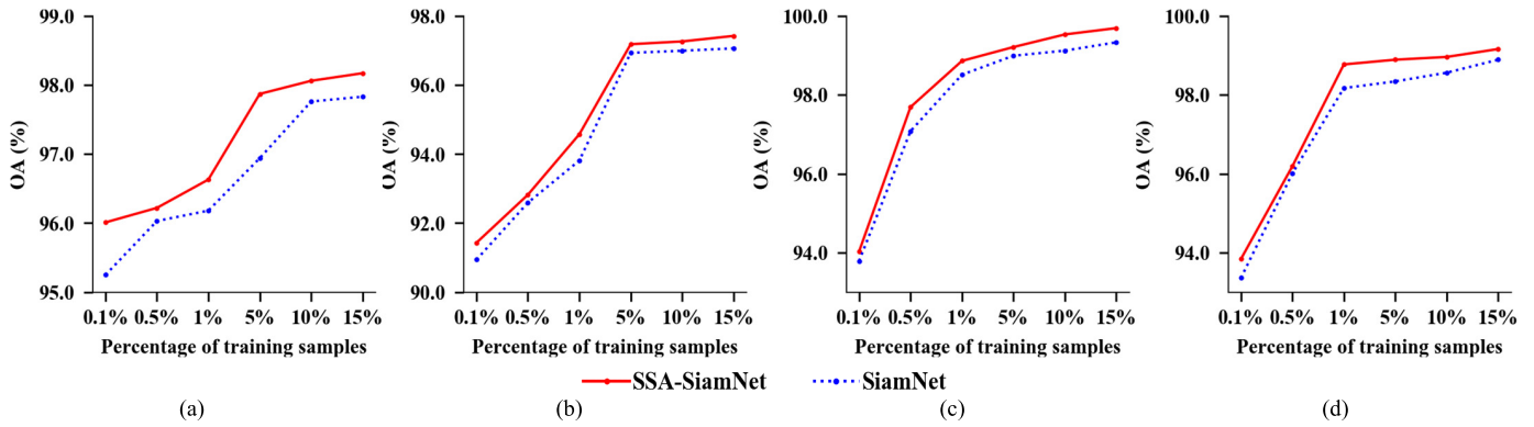
Fig. 12. Accuracy (in terms of OA) of SSA-SiamNet and SiamNet with different proportions of training samples. (a) Farmland dataset. (b) River dataset. (c) Santa Barbara dataset. (d) Bay Area dataset.
