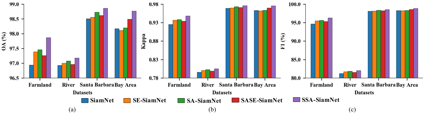
Fig. 8. Accuracy of the SiamNet with different attention modules for all four datasets. (a) OA. (b) Kappa. (c) F1-Score.
