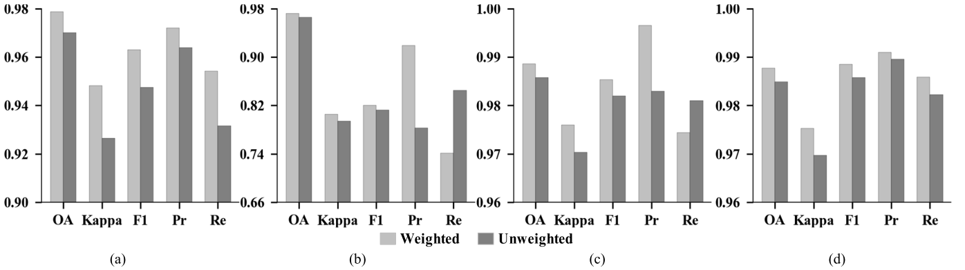
Fig. 9. Accuracy of the loss function and weighted loss function for the four datasets. (a) Farmland dataset. (b) River dataset. (c) Santa Barbara dataset. (d) Bay Area dataset.
