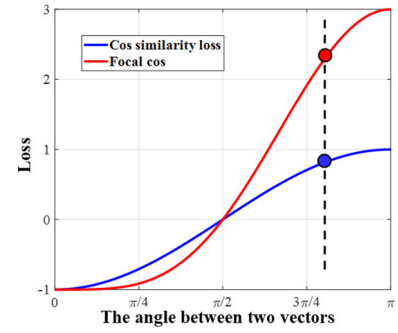
Fig. 4. Comparison of cos similarity loss function in blue and proposed focal cos loss function in red.
