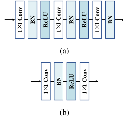
Fig. 3. Architecture of: (a) projector and (b) predictor.
