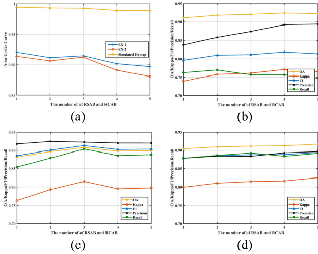
Fig. 15. HACD-task result and HBCD results regard to the number of RSAB and RCAB in the SSA module: (a) AUC performance for three datasets; the five quantitative evaluation indices (OA, Kappa, F1, Precision, and Recall) on the binary change detection results on: (b) Hermiston dataset; (c) Bay dataset; and (d) Santa Barbara dataset.
