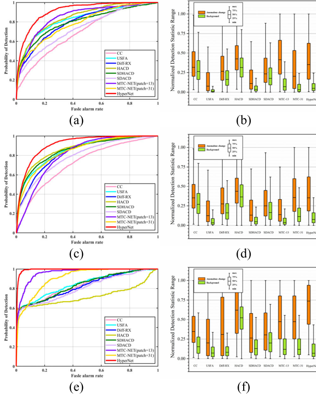
Fig. 11. First column is the ROC curves of all methods on: (a) EX-1: D1F12H1-D1F12H2; (c) EX-2: D1F12H1-D2F22H2; and (e) simulated Hymap dataset, and the second column is separability maps of all methods on: (b) EX-1: D1F12H1-D1F12H2; (d) EX-2: D1F12H1-D2F22H2; and (f) simulated Hymap dataset.
