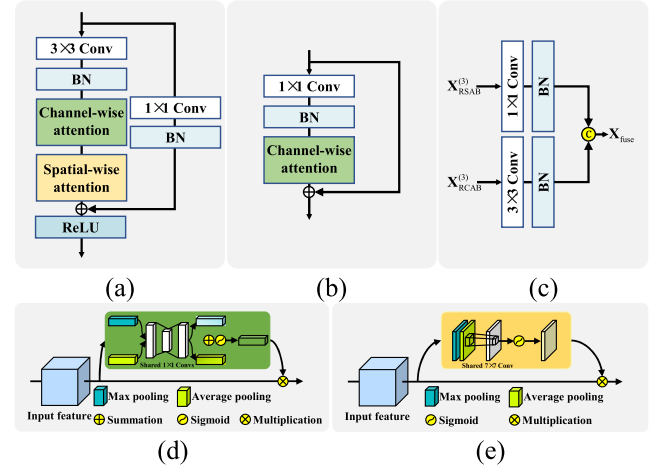
Fig. 2. Architecture of: (a) RSAB; (b) RCAB; (c) adaptive feature fusion block; (d) CA; and (e) SA.
