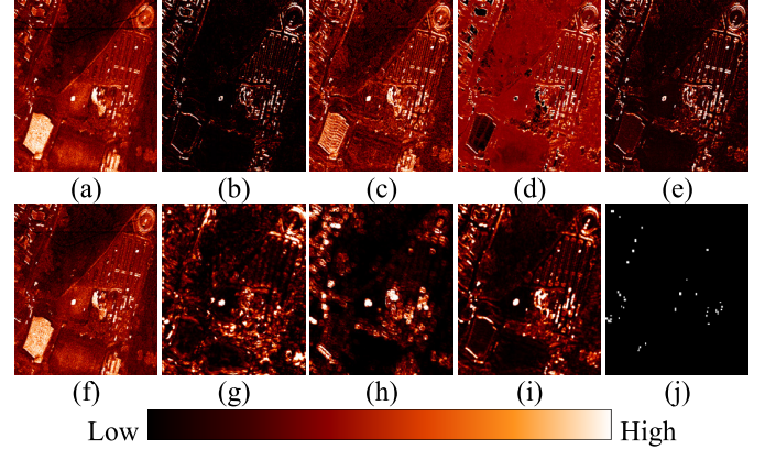
Fig. 8. Anomalous change detection maps of EX-1: D1F12H1-D1F12H2 on: (a) CC; (b) USFA; (c) Diff_RX; (d) HACD; (e) SDHACD; (f) SDACD; (g) MTC-NET (patch = 13); (h) MTC-NET (patch = 31); (i) proposed HyperNet; and (j) reference change map.
