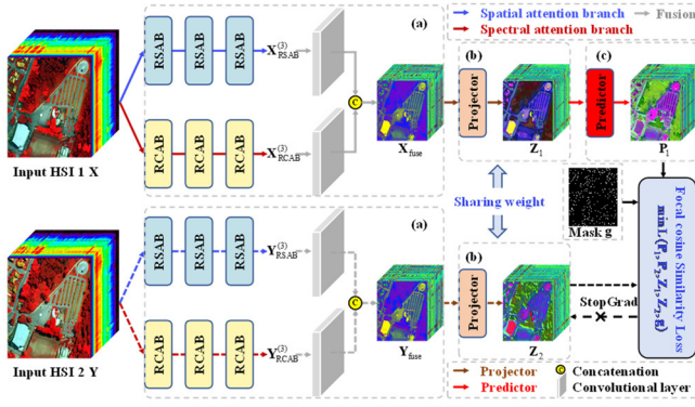
Fig. 1. Structure of the proposed HyperNet for hyperspectral change detection: (a) is the SSA module, which is especially designed to fully exploit the abundant information of HSIs, including the RSABs, RCABs, and the fusion block; (b) is the projector to improve the nonlinear feature mapping ability; and (c) is the predictor, which is only assembled on one of the branches of the HyperNet and is swapped for another branch to alternatively minimize the similarity loss.
