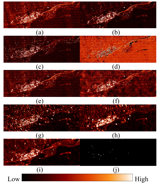
Fig. 10. Anomalous change detection maps of simulated Hymap dataset on: (a) CC; (b) USFA; (c) Diff_RX; (d) HACD; (e) SDHACD; (f) SDACD; (g) MTC-NET (patch = 13); (h) MTC-NET (patch = 31); (i) proposed HyperNet; and (j) reference change map.
