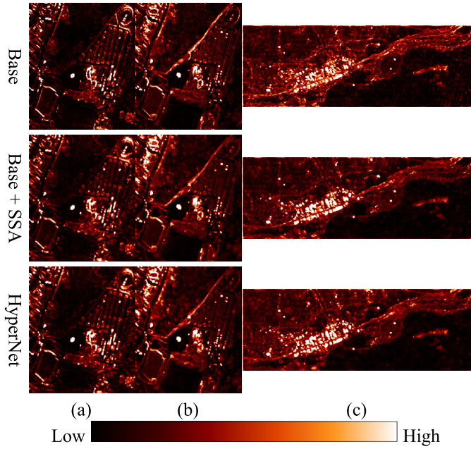
Fig. 18. Anomalous change detection map comparison of ablation experiments of: (a) EX1: D1F12H1-D1F12H2; (b) EX-2: D1F12H1-D2F22H2; and (c) simulated Hymap dataset. (From top to bottom) Result from Base, Base + SSA, and HyperNet.
