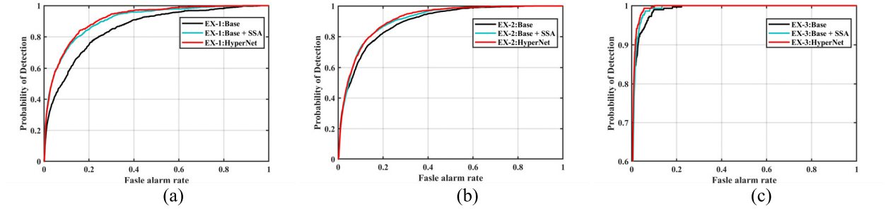
Fig. 17. ROC comparison of ablation experiments of HyperNet on three HACD-task datasets of: (a) EX1: D1F12H1-D1F12H2; (b) EX-2: D1F12H1-D2F22H2; and (c) simulated Hymap dataset.
