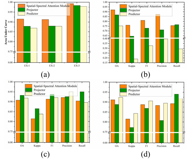
Fig. 16. Evaluation of the performance of the representation from SSA module, projector, and predictor for HACD-task and HBCD tasks: (a) AUC performance for three datasets of HACD-task; the five quantitative evaluation indices (OA, Kappa, F1, Precision, and Recall) of HBCD on: (b) Hermiston dataset; (c) Bay dataset; and (d) Santa Barbara dataset.
