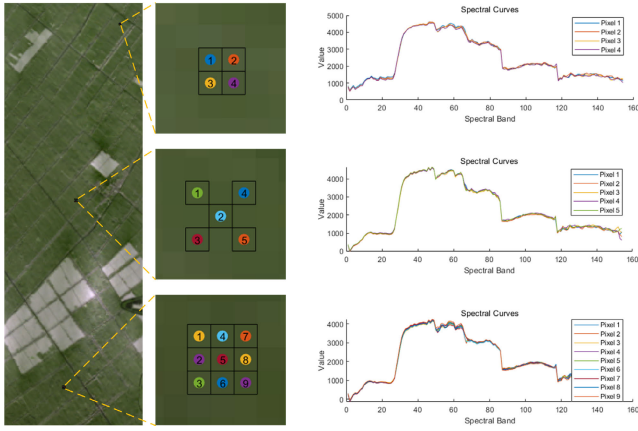
Fig. 2. Spectral similarity of neighboring pixels in hyperspectral images.
