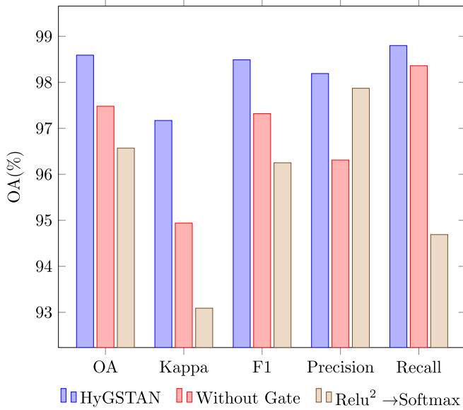
Fig. 13. HyGSTAN ablation experiments and results under different settings on the Bay Area dataset.
