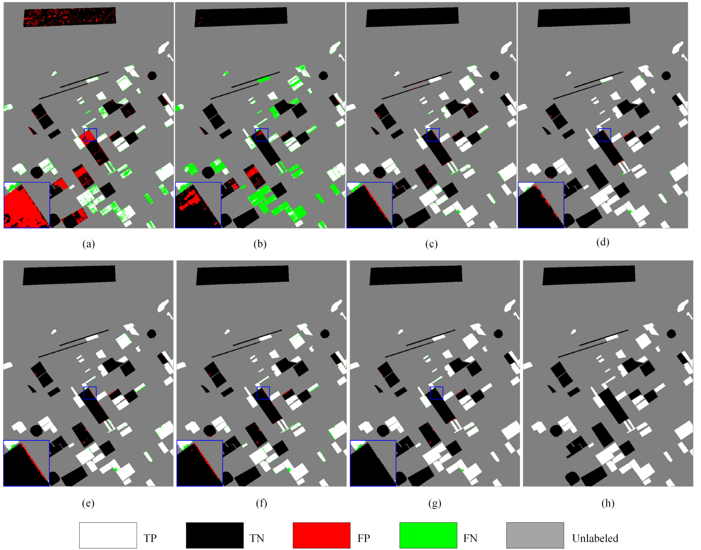
Fig. 11. CD maps for the Santa Barbara dataset. (a) CVA. (b) DPCA. (c) BIT. (d) CSA-Net. (e) ML-EDAN. (f) SST-Former. (g) Ours. (h) Ground truth.
