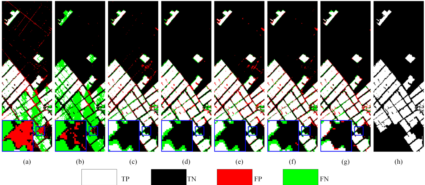
Fig. 10. CD maps for the Farmland dataset. (a) CVA. (b) DPCA. (c) BIT. (d) CSA-Net. (e) ML-EDAN. (f) SST-Former. (g) Ours. (h) Ground truth.
