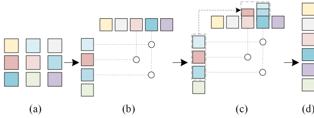
Fig. 3. Spectral similarity filtering module. (a) Original spectral vector input. (b) Extraction of index pairs for similar spectral vectors. (c) Averaging process for similar spectral pairs. (d) Resulting merged spectral vector.
