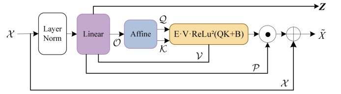
Fig. 4. Architecture of the \text{GS}^2\text{AM} .
