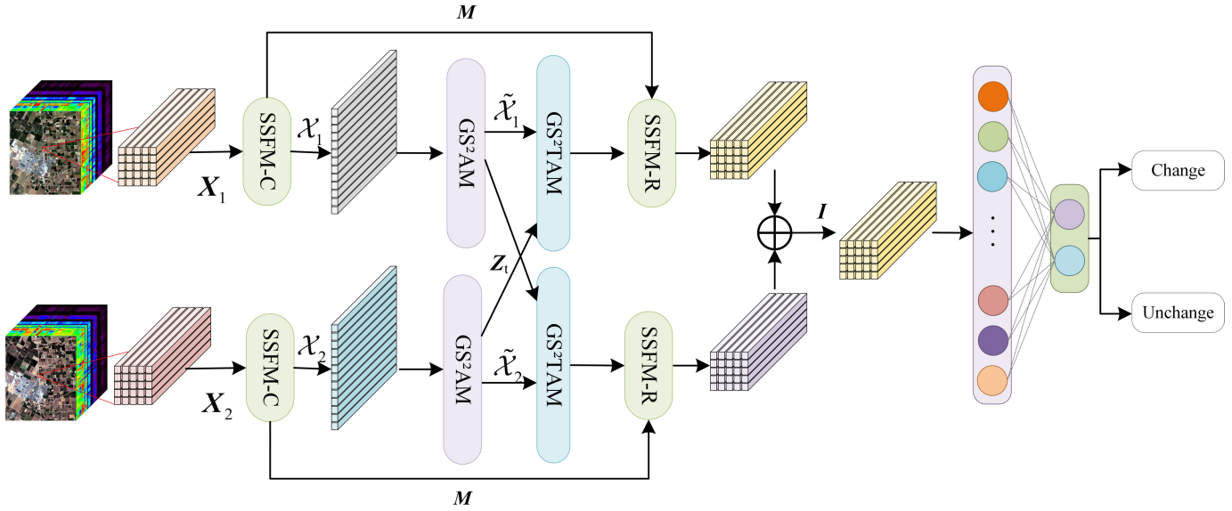
Fig. 1. Architecture of the proposed HyGSTAN for hyperspectral image CD.
