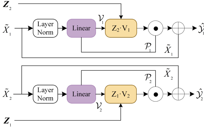
Fig. 5. Architecture of the GS²TAM.
