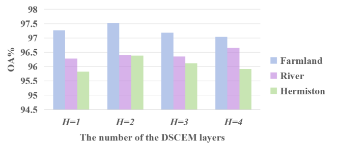
Fig. 9. OA versus the number of DSCem layers.
