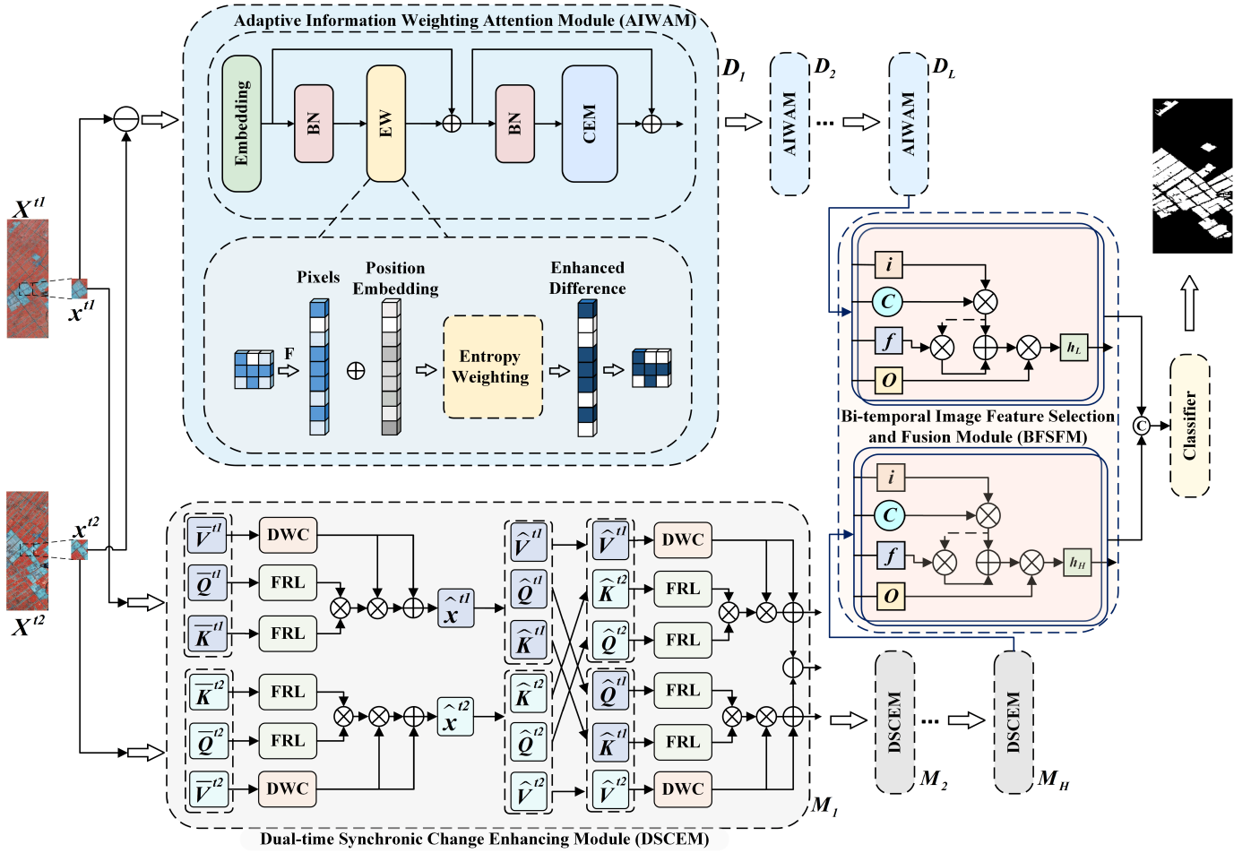
Fig. 1. Framework of the proposed AIWSEN for HSI CD includes AIWAM, DSCEM, and BFSFM. The AIWAM enhances the difference features, the DSCEM extracts the interactive features, and the BFSFM fuses the extracted features.
