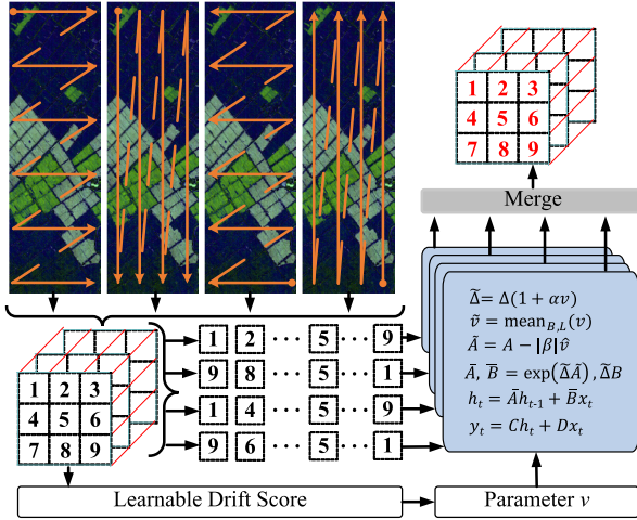
Fig. 3. TA-SS2D operation. The input feature map is scanned along four directions—(left-to-right), (right-to-left), (top-to-bottom), and (bottom-to-top)—to generate directional sequential representations. These sequences are then processed to capture long-range dependencies. Finally, the outputs from all directions are fused to produce the final feature representation.
