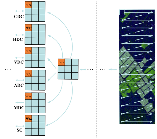
Fig. 4. Kernel reparameterization process of LDSM. CDC, HDC, VDC, ADC, MDC, and SC are parameterized into structured 3 \times 3 kernels and fused into a unified kernel w . The fused kernel scans the input feature map, and gradients are backpropagated to update the parameters of all six convolution branches.
