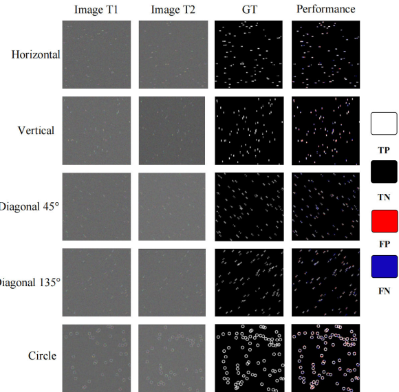
Fig. 11. CD results on synthetic datasets with five change orientations.
