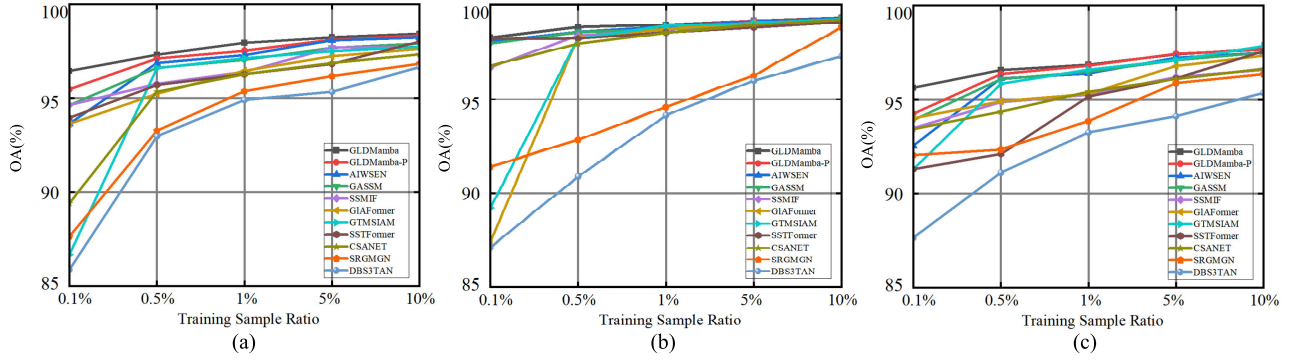
Fig. 12. CD performance of different methods under different training sample ratios. (a) Farmland. (b) Hermiston. (c) River.
