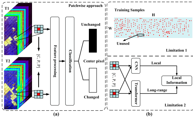
Fig. 1. Patch-based processing and its limitations. (a) Patch-based framework. (b) Limitations.
