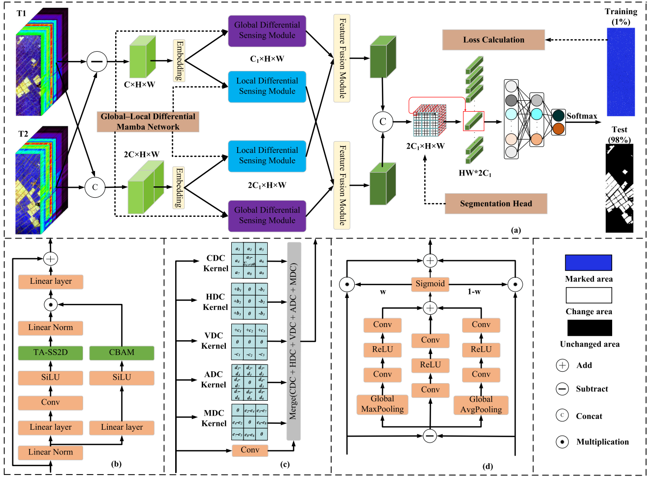
Fig. 2. Overview of the proposed GLDMamba framework for image-level HSI-CD. The final output is a change map, where white pixels represent the changed areas. (a) GLDMamba framework. (b) GDSM. (c) LDSM. (d) FFM.
