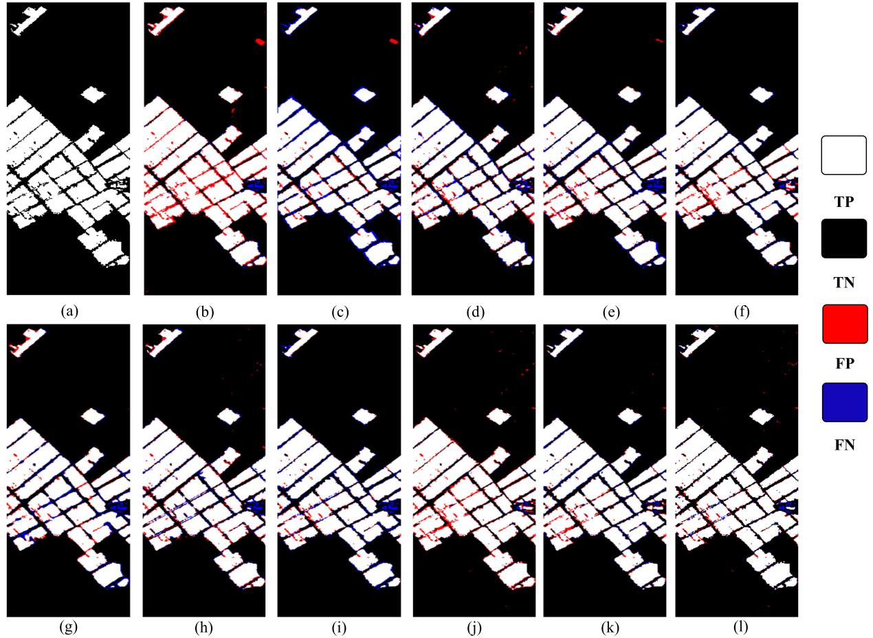
Fig. 8. CD results on the Farmland dataset. (a) GT. (b) DBS3TAN. (c) SRGMGN. (d) CSANet. (e) SSTFormer. (f) GTMSiam. (g) GLAFormer. (h) SSMIF. (i) GASSM. (j) AIWSEN. (k) GLDMamba-P. (l) GLDMamba.
