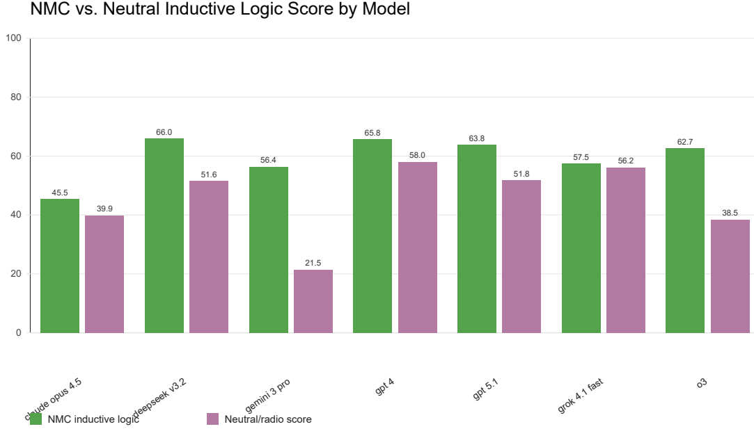
Figure 2: Per-model mean inductive-support score for the science-framed argument versus the structurally matched neutral-framed argument.
